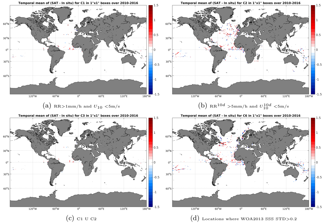
Figure 12: Temporal mean gridded over spatial boxes of size 1^\circ \times 1^\circ of \Delta SSS (SMOS-L2-DPGS-v662 - TSG-GOSUD-Research-vessel) for 4 different subdatasets corresponding to: RR > 1 mm/h and U_{10} < 5 m/s (a), RR^{10d} > 5 mm/h and U_{10}^{10d} < 5 m/s (b), C1 U C2 (c), Locations where WOA2013 SSS STD > 0.2 (d).
