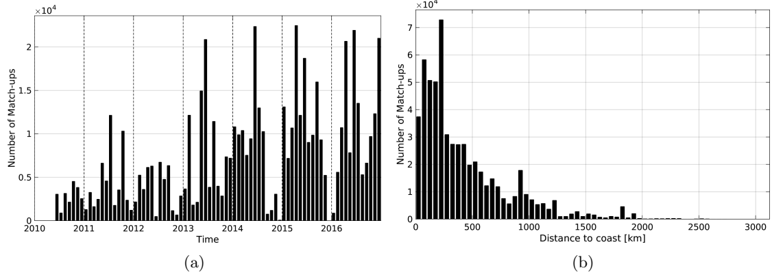
Figure 1: Number of match-ups between TSG-GOSUD-Research-vessel and SMOS-L2-DPGS-v662 SSS as a function of time (a) and as function of the distance to coast (b) over the Global Ocean Pi-MEP region and for the full satellite product period.
