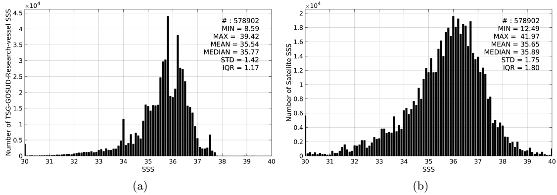
Figure 2: Histograms of SSS from TSG-GOSUD-Research-vessel (a) and SMOS-L2-DPGS-v662 (b) considering all match-up pairs per bins of 0.1 over the Global Ocean Pi-MEP region and for the full satellite product period.
