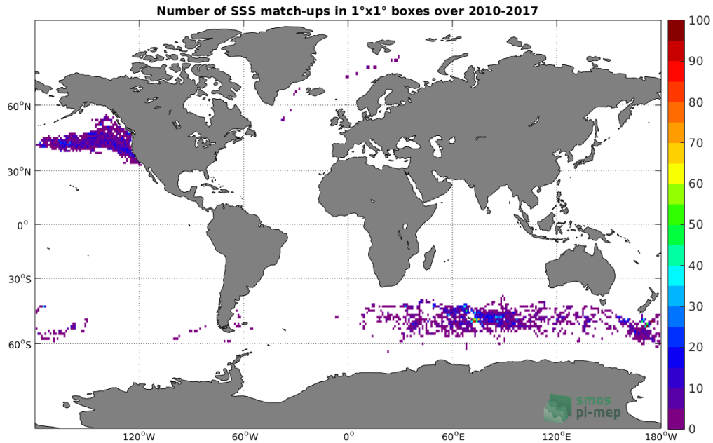
Figure 4: Number of SSS match-ups between Sea mammals SSS and the SMOS SSS L2 v662 (ESA) SSS product for the Global Ocean Pi-MEP region over 1^\circ \times 1^\circ boxes and for the full satellite product period.
