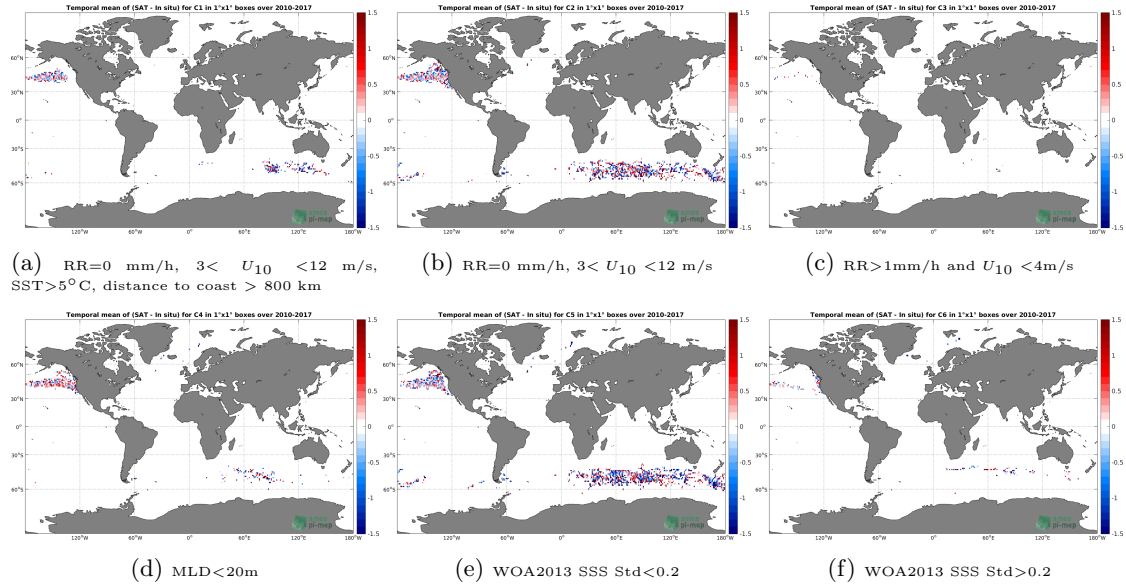
Figure 12: Temporal mean gridded over spatial boxes of size 1^\circ \times 1^\circ of \Delta SSS (SMOS SSS L2 v662 (ESA) - Sea mammals) for 6 different subdatasets corresponding to: RR=0 mm/h, 3 < U_{10} < 12 m/s, SST >5^\circ\text{C} , distance to coast > 800 km (a), RR=0 mm/h, 3 < U_{10} < 12 m/s (b), RR >1 mm/h and U_{10} < 4 m/s (c), MLD <20 m (d), WOA2013 SSS Std <0.2 (e), WOA2013 SSS Std >0.2 (f).
