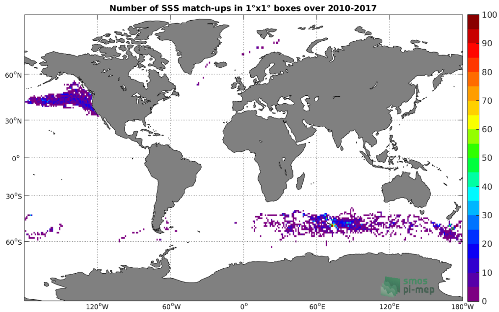
Figure 4: Number of SSS match-ups between Sea mammals SSS and the SMOS SSS L2 v662 (ESA) SSS product for the Global Ocean Pi-MEP region over 1°x1° boxes and for the full satellite product period.
