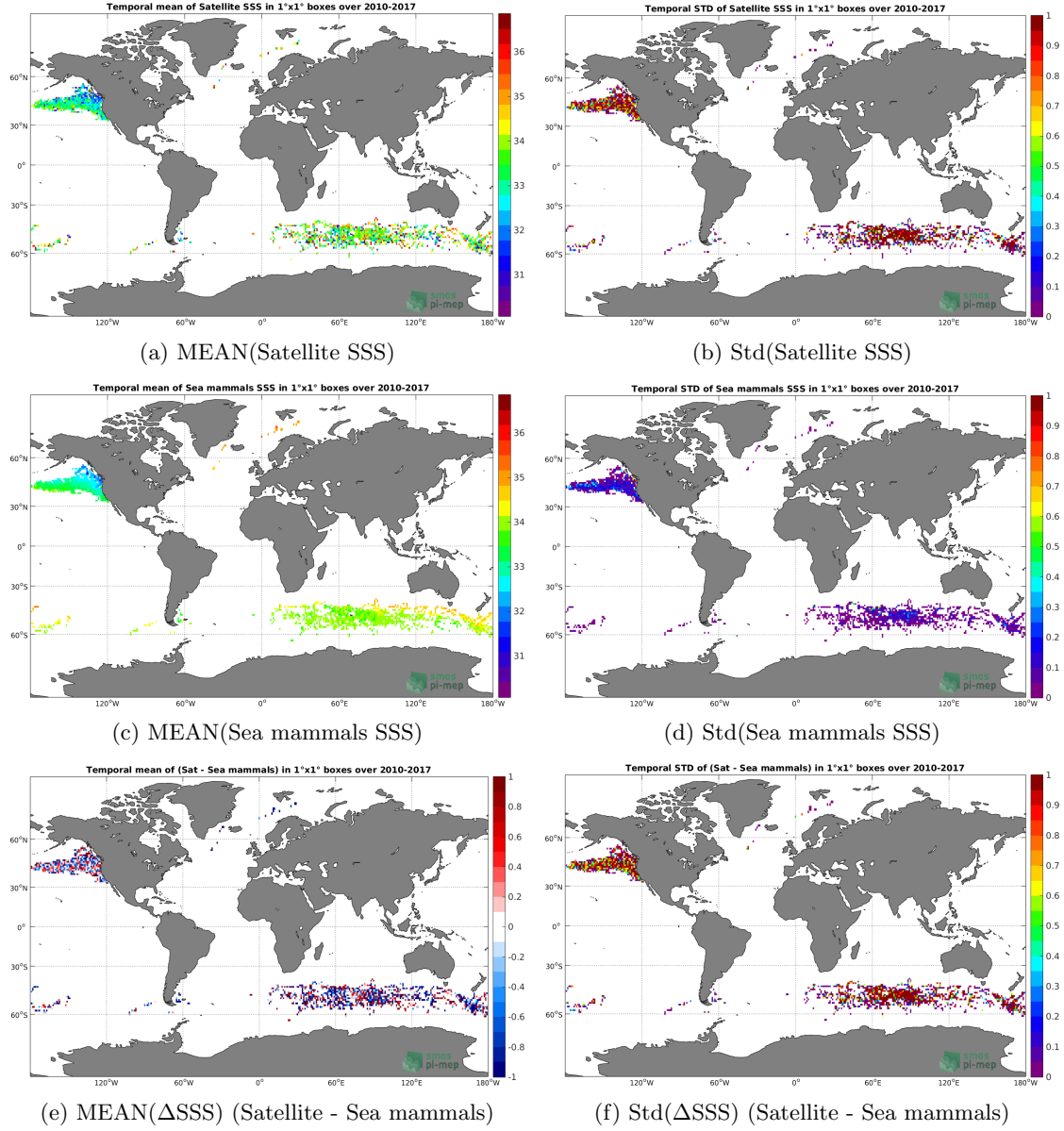
Figure 6: Temporal mean (left) and Std (right) of SSS from SMOS SSS L2 v662 (ESA) (top), Sea mammals (middle), and of \Delta SSS (Satellite - Sea mammals). Only match-up pairs are used to generate these maps.
