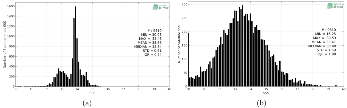
Figure 2: Histograms of SSS from Sea mammals (a) and SMOS SSS L2 v662 (ESA) (b) considering all match-up pairs per bins of 0.1 over the Global Ocean Pi-MEP region and for the full satellite product period.
