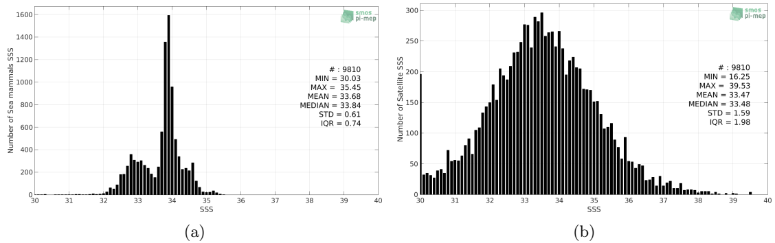
Figure 2: Histograms of SSS from Sea mammals (a) and SMOS L2 v662 (ESA) (b) considering all match-up pairs per bins of 0.1 over the Global Ocean Pi-MEP region and for the full satellite product period.
