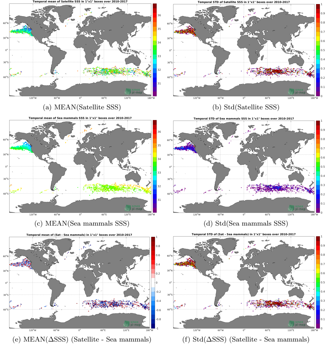
Figure 6: Temporal mean (left) and Std (right) of SSS from SMOS L2 v662 (ESA) (top), Sea mammals (middle), and of \Delta SSS (Satellite - Sea mammals). Only match-up pairs are used to generate these maps.
