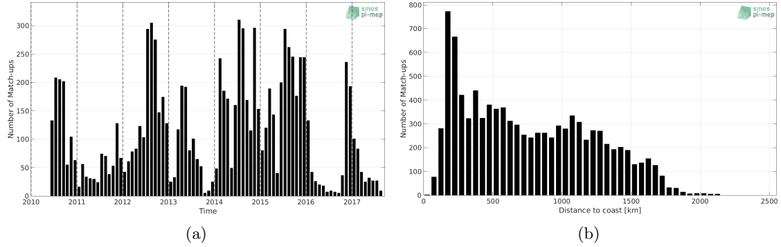
Figure 1: Number of match-ups between Sea mammals and SMOS L2 v662 (ESA) SSS as a function of time (a) and as function of the distance to coast (b) over the Global Ocean Pi-MEP region and for the full satellite product period.
