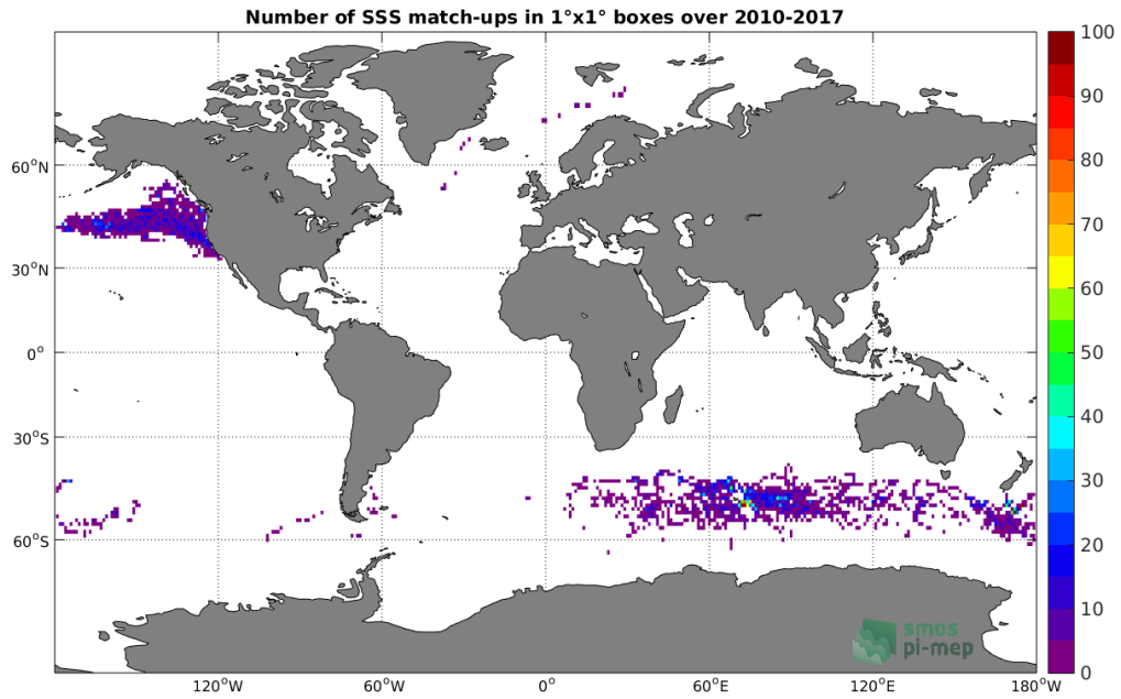
Figure 4: Number of SSS match-ups between Sea mammals SSS and the SMOS L2 v662 (ESA) SSS product for the Global Ocean Pi-MEP region over 1°x1° boxes and for the full satellite product period.
