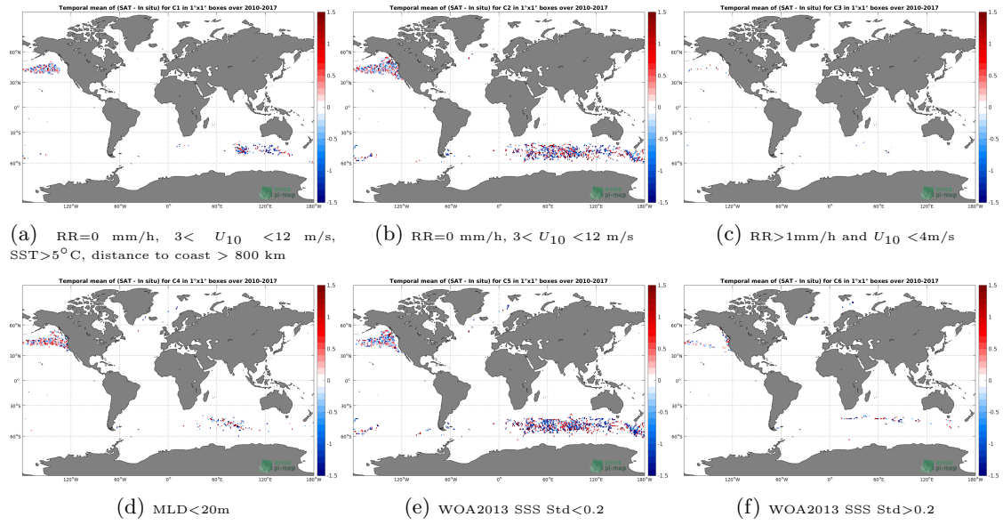
Figure 12: Temporal mean gridded over spatial boxes of size 1^\circ \times 1^\circ of \Delta SSS (SMOS L2 v662 (ESA) - Sea mammals) for 6 different subdatasets corresponding to: RR=0 mm/h, 3 < U_{10} < 12 m/s, SST > 5^\circ C , distance to coast > 800 km (a), RR=0 mm/h, 3 < U_{10} < 12 m/s (b), RR > 1 mm/h and U_{10} < 4 m/s (c), MLD < 20 m (d), WOA2013 SSS Std < 0.2 (e), WOA2013 SSS Std > 0.2 (f).
