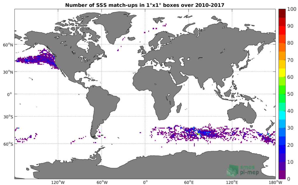
Figure 4: Number of SSS match-ups between Sea mammals SSS and the SMOS-L2-DPGS-v662 SSS product for the Global Ocean Pi-MEP region over 1^\circ \times 1^\circ boxes and for the full satellite product period.
