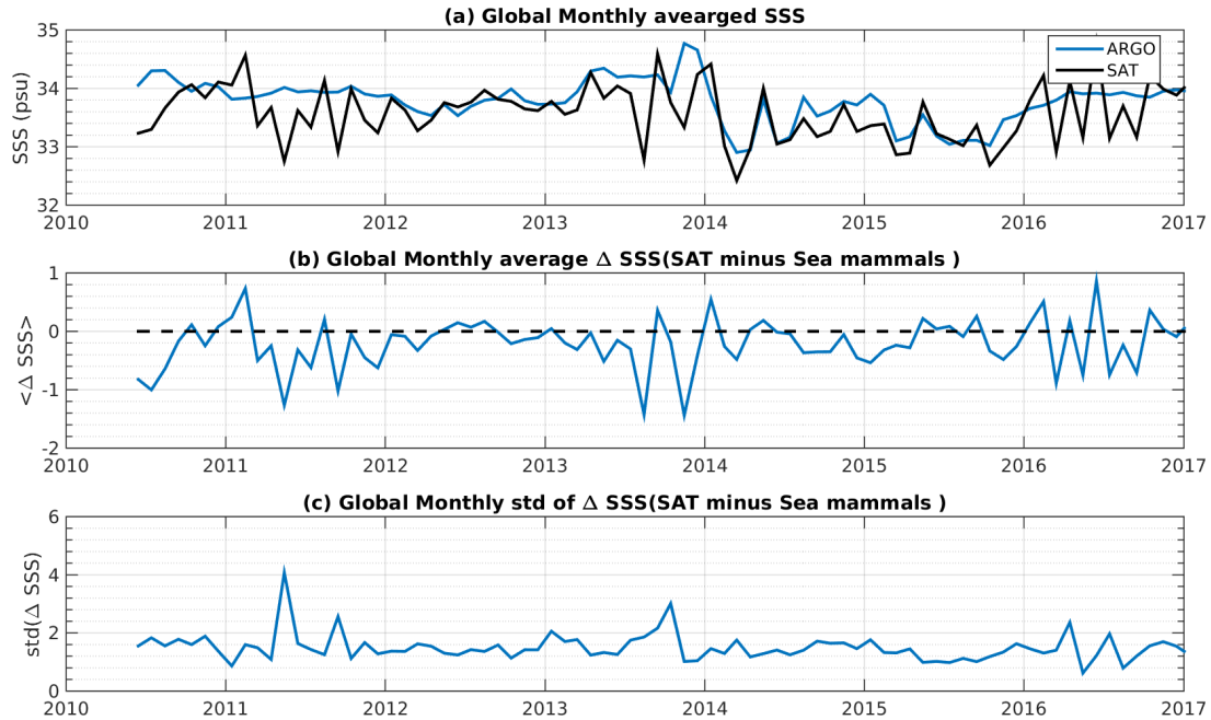
Figure 7: Time series of the monthly averaged mean SSS (top), mean \Delta SSS (Satellite - Sea mammals) and STD of \Delta SSS (Satellite - Sea mammals) over the Global Ocean Pi-MEP region considering all match-ups collected by the Pi-MEP platform.
