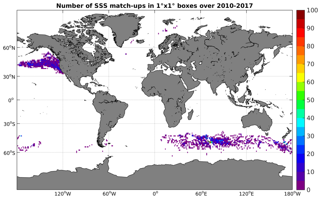
Figure 4: Number of SSS match-ups between Sea mammals SSS and the SMOS-L2-DPGS-v662 SSS product for the Global Ocean Pi-MEP region over 1^\circ \times 1^\circ boxes and for the full satellite product period.
