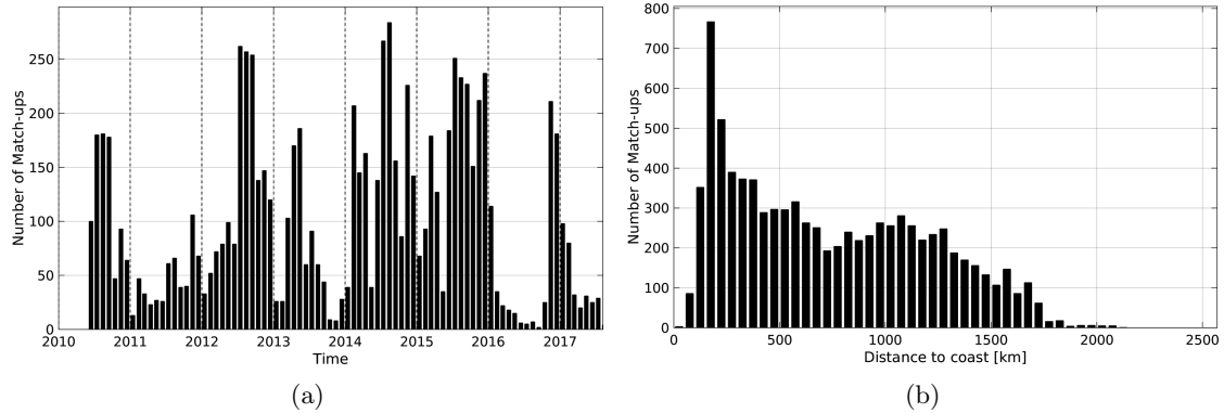
Figure 1: Number of match-ups between Sea mammals and SMOS-L2-DPGS-v662 SSS as a function of time (a) and as function of the distance to coast (b) over the Global Ocean Pi-MEP region and for the full satellite product period.
