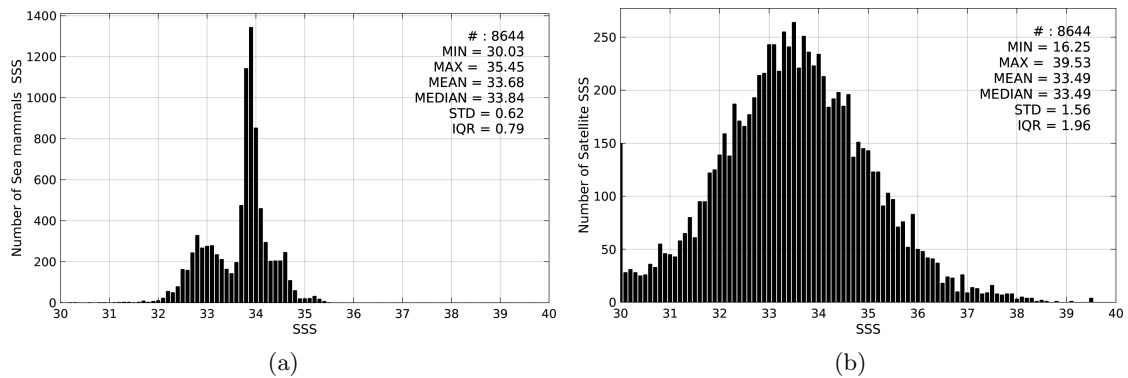
Figure 2: Histograms of SSS from Sea mammals (a) and SMOS-L2-DPGS-v662 (b) considering all match-up pairs per bins of 0.1 over the Global Ocean Pi-MEP region and for the full satellite product period.
