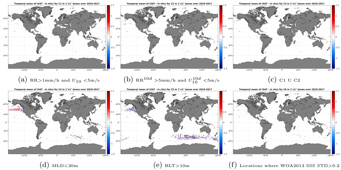
Figure 12: Temporal mean gridded over spatial boxes of size 1^\circ \times 1^\circ of \Delta SSS (SMOS-L2-DPGS-v662 - Sea mammals) for 6 different subdatasets corresponding to: RR > 1\text{mm/h} and U_{10} < 5\text{m/s} (a), RR^{10d} > 5\text{mm/h} and U_{10}^{10d} < 5\text{m/s} (b), C1 U C2 (c), MLD < 20\text{m} (d), BLT > 10\text{m} (e), Locations where WOA2013 SSS STD > 0.2 (f).
