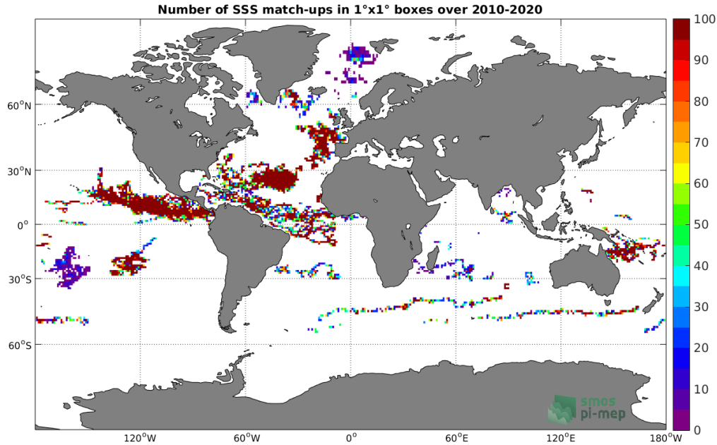
Figure 3: Number of SSS match-ups between Surface drifters SSS and the SMOS SSS L2 v662 (ESA) SSS product for the Global Ocean Pi-MEP region over 1^\circ \times 1^\circ boxes and for the full satellite product period.
