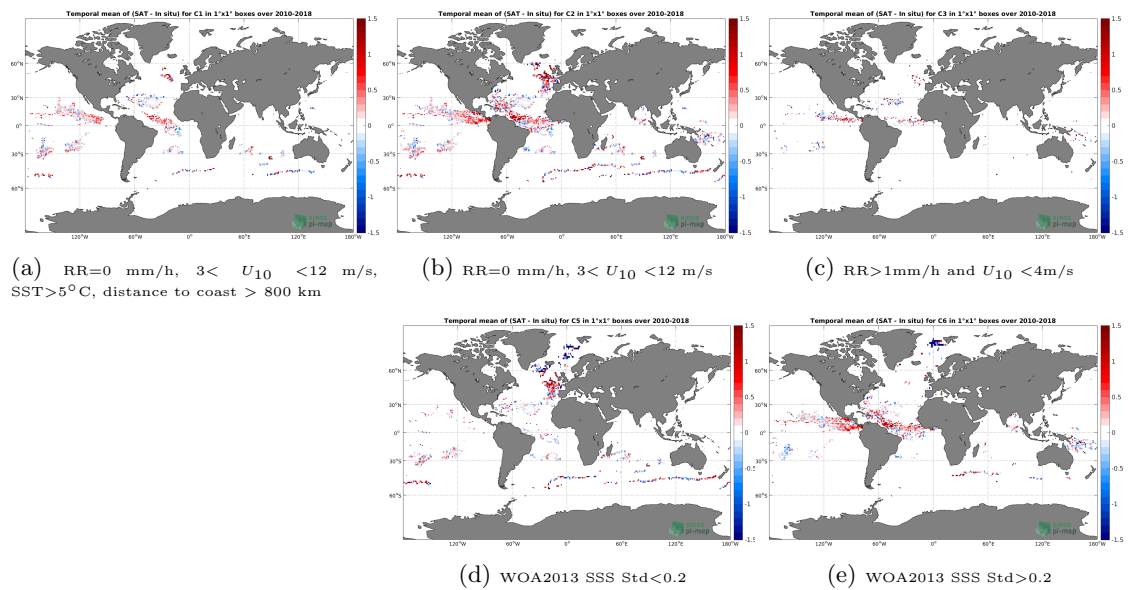
Figure 11: Temporal mean gridded over spatial boxes of size 1^\circ \times 1^\circ of \Delta SSS (SMOS SSS L2 v662 (ESA) - Surface drifters) for 5 different subdatasets corresponding to:RR=0 mm/h, 3 < U_{10} < 12 m/s, SST >5^\circ\text{C} , distance to coast > 800 km (a), RR=0 mm/h, 3 < U_{10} < 12 m/s (b), RR >1 mm/h and U_{10} < 4 m/s (c), WOA2013 SSS Std <0.2 (d), WOA2013 SSS Std >0.2 (e).
