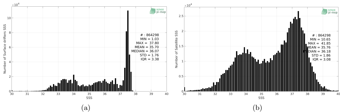
Figure 2: Histograms of SSS from Surface drifters (a) and SMOS SSS L2 v662 (ESA) (b) considering all match-up pairs per bins of 0.1 over the Global Ocean Pi-MEP region and for the full satellite product period.
