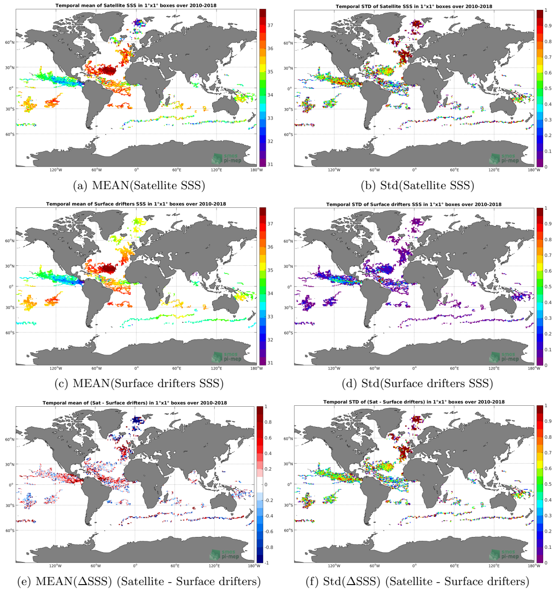
Figure 5: Temporal mean (left) and Std (right) of SSS from SMOS SSS L2 v662 (ESA) (top), Surface drifters (middle), and of \Delta SSS (Satellite - Surface drifters). Only match-up pairs are used to generate these maps.
