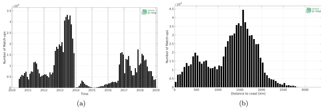
Figure 1: Number of match-ups between Surface drifters and SMOS SSS L2 v662 (ESA) SSS as a function of time (a) and as function of the distance to coast (b) over the Global Ocean Pi-MEP region and for the full satellite product period.
