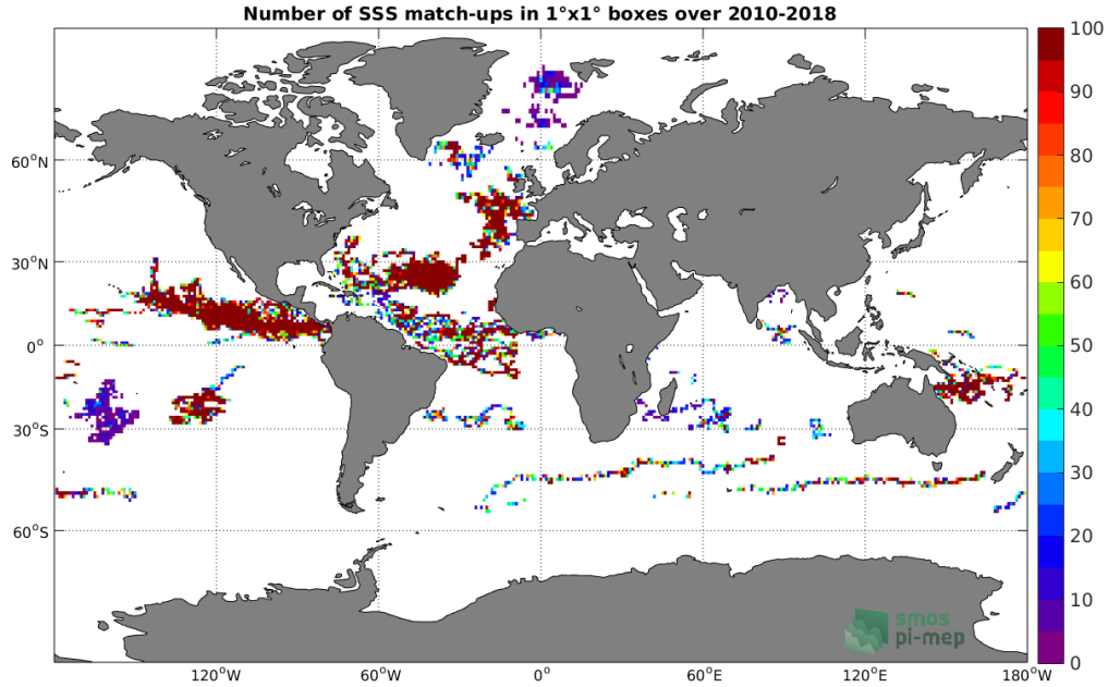
Figure 3: Number of SSS match-ups between Surface drifters SSS and the SMOS SSS L2 v662 (ESA) SSS product for the Global Ocean Pi-MEP region over 1°x1° boxes and for the full satellite product period.
