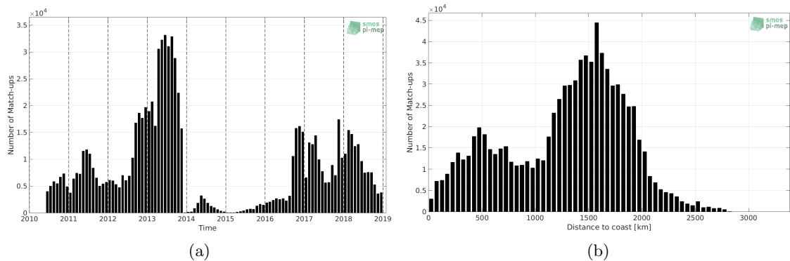
Figure 1: Number of match-ups between Surface drifters and SMOS L2 v662 (ESA) SSS as a function of time (a) and as function of the distance to coast (b) over the Global Ocean Pi-MEP region and for the full satellite product period.
