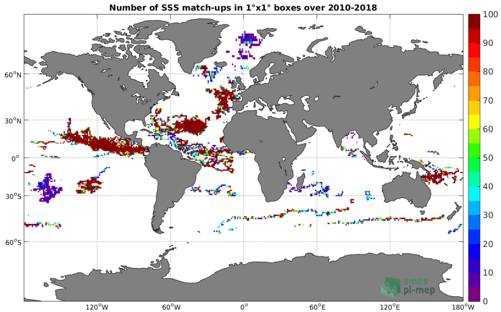
Figure 3: Number of SSS match-ups between Surface drifters SSS and the SMOS L2 v662 (ESA) SSS product for the Global Ocean Pi-MEP region over 1°x1° boxes and for the full satellite product period.
