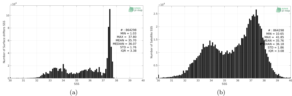
Figure 2: Histograms of SSS from Surface drifters (a) and SMOS L2 v662 (ESA) (b) considering all match-up pairs per bins of 0.1 over the Global Ocean Pi-MEP region and for the full satellite product period.
