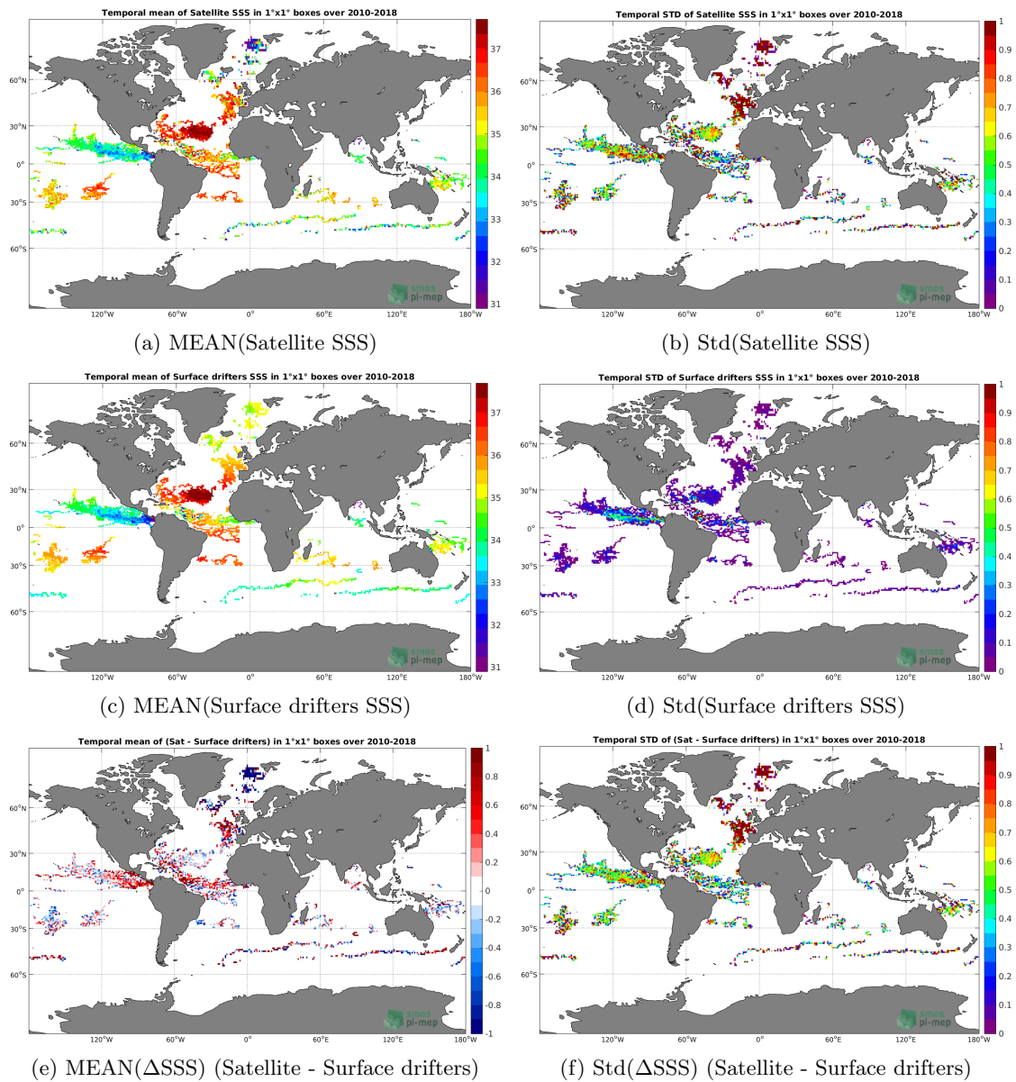
Figure 5: Temporal mean (left) and Std (right) of SSS from SMOS L2 v662 (ESA) (top), Surface drifters (middle), and of \Delta SSS (Satellite - Surface drifters). Only match-up pairs are used to generate these maps.
