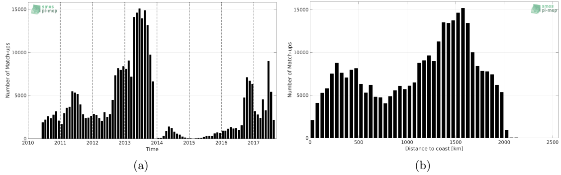
Figure 1: Number of match-ups between Surface drifters and SMOS-L2-DPGS-v662 SSS as a function of time (a) and as function of the distance to coast (b) over the Global Ocean Pi-MEP region and for the full satellite product period.
