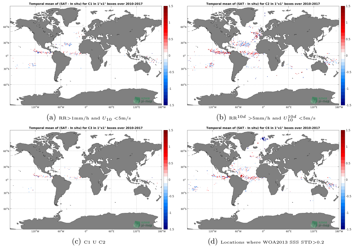
Figure 11: Temporal mean gridded over spatial boxes of size 1^\circ \times 1^\circ of \Delta SSS (SMOS-L2-DPGS-v662 - Surface drifters) for 4 different subdatasets corresponding to: RR > 1\text{mm/h} and U_{10} < 5\text{m/s} (a), RR^{10d} > 5\text{mm/h} and U_{10}^{10d} < 5\text{m/s} (b), C1 U C2 (c), Locations where WOA2013 SSS STD > 0.2 (d).
