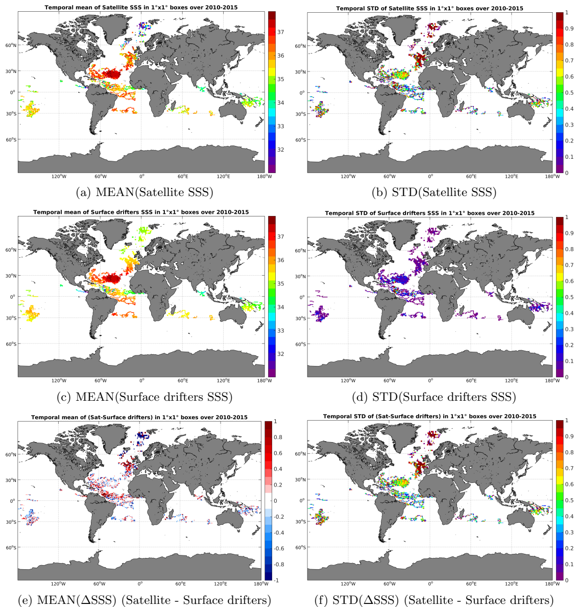
Figure 5: Temporal mean (left) and STD (right) of SSS from SMOS-L2-DPGS-v662 (top), Surface drifters (middle), and of \Delta SSS (Satellite - Surface drifters). Only match-up pairs are used to generate these maps.
