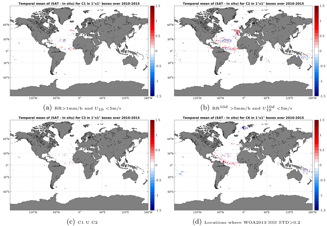
Figure 11: Temporal mean gridded over spatial boxes of size 1^\circ \times 1^\circ of \Delta SSS (SMOS-L2-DPGS-v662 - Surface drifters) for 4 different subdatasets corresponding to: RR > 1mm/h and U_{10} < 5\text{m/s} (a), RR^{10d} > 5\text{mm/h} and U_{10}^{10d} < 5\text{m/s} (b), C1 U C2 (c), Locations where WOA2013 SSS STD > 0.2 (d).
