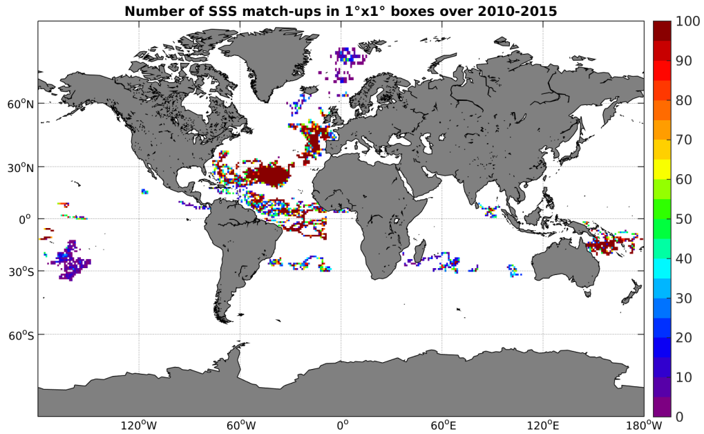
Figure 3: Number of SSS match-ups between Surface drifters SSS and the SMOS-L2-DPGS-v662 SSS product for the Global Ocean Pi-MEP region over 1°x1° boxes and for the full satellite product period.
