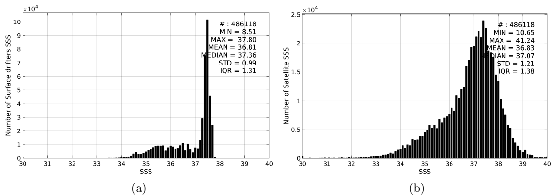
Figure 2: Histograms of SSS from Surface drifters (a) and SMOS-L2-DPGS-v662 (b) considering all match-up pairs per bins of 0.1 over the Global Ocean Pi-MEP region and for the full satellite product period.
