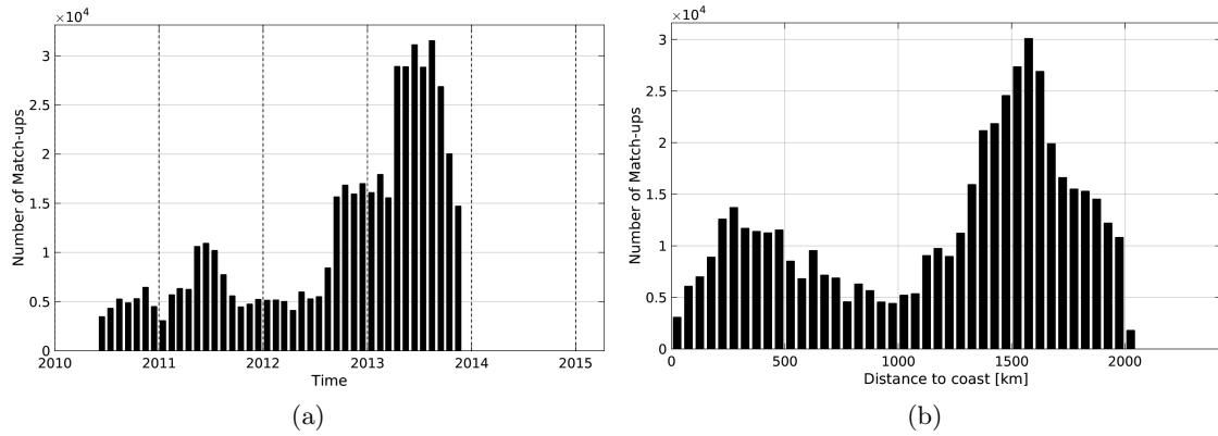
Figure 1: Number of match-ups between Surface drifters and SMOS-L2-DPGS-v662 SSS as a function of time (a) and as function of the distance to coast (b) over the Global Ocean Pi-MEP region and for the full satellite product period.
