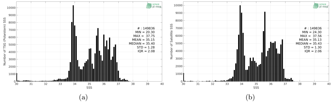
Figure 2: Histograms of SSS from TSG (Polarstern) (a) and SMAP SSS L4 OI v1 - 7 Days (IPRC) (b) considering all match-up pairs per bins of 0.1 over the Global Ocean Pi-MEP region and for the full satellite product period.
