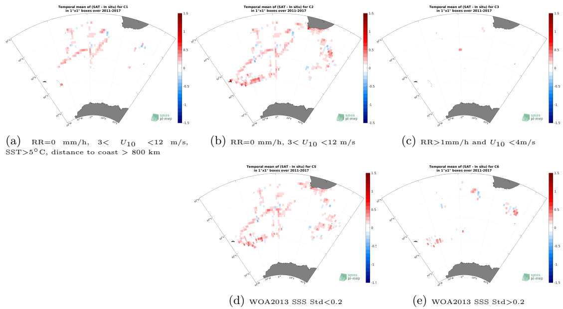
Figure 12: Temporal mean gridded over spatial boxes of size 1^\circ \times 1^\circ of \Delta SSS (SMAP SSS L4 OI v1 - 7 Days (IPRC) - TSG (NCEI-0170743)) for 5 different subdatasets corresponding to:RR=0 mm/h, 3 < U_{10} < 12 m/s, SST >5^\circ C, distance to coast > 800 km (a), RR=0 mm/h, 3 < U_{10} < 12 m/s (b), RR >1 mm/h and U_{10} < 4 m/s (c), WOA2013 SSS Std <0.2 (d), WOA2013 SSS Std >0.2 (e).
