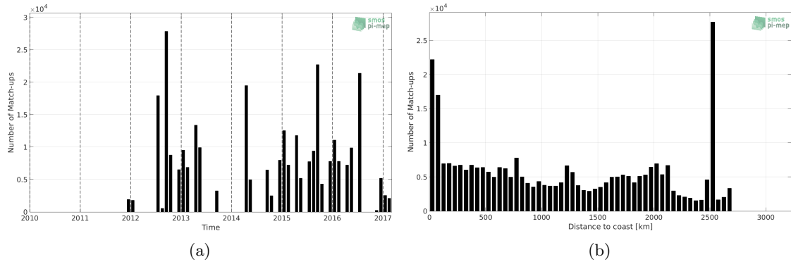
Figure 1: Number of match-ups between TSG (NCEI-0170743) and SMAP SSS L4 OI v1 - 7 Days (IPRC) SSS as a function of time (a) and as function of the distance to coast (b) over the Global Ocean Pi-MEP region and for the full satellite product period.
