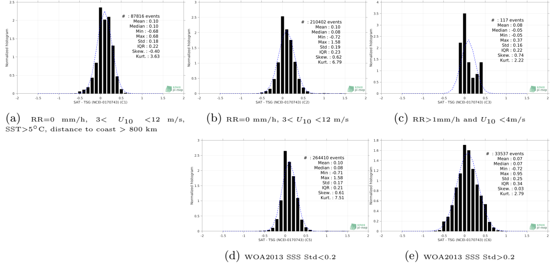
Figure 13: Normalized histogram of \Delta SSS (SMAP SSS L4 OI v1 - 7 Days (IPRC) - TSG (NCEI-0170743)) for 5 different subdatasets corresponding to: RR=0 mm/h, 3 < U_{10} < 12 m/s, SST>5°C, distance to coast > 800 km (a), RR=0 mm/h, 3 < U_{10} < 12 m/s (b), RR>1mm/h and U_{10} < 4 m/s (c), WOA2013 SSS Std<0.2 (d), WOA2013 SSS Std>0.2 (e).
