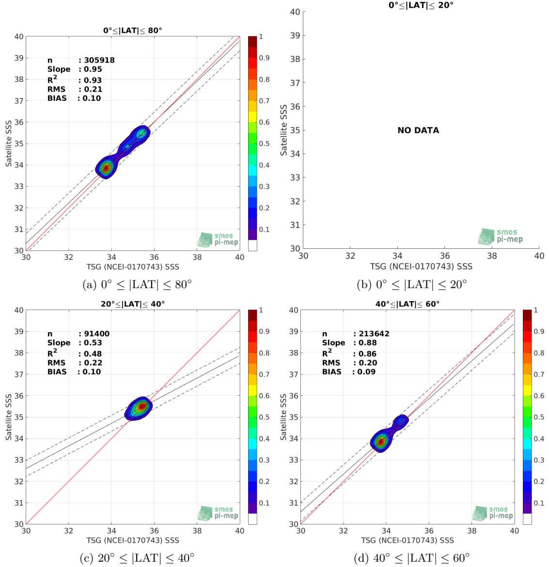
Figure 9: Contour maps of the concentration of SMAP SSS L4 OI v1 - 7 Days (IPRC) SSS (y-axis) versus TSG (NCEI-0170743) SSS (x-axis) at match-up pairs for different latitude bands. For each plot, the red line shows x=y . The black thin and dashed lines indicate a linear fit through the data cloud and the \pm 95\% confidence levels, respectively. The number match-up pairs n , the slope and R^2 coefficient of the linear fit, the root mean square (RMS) and the mean bias between satellite and in situ data are indicated for each latitude band in each plots.
