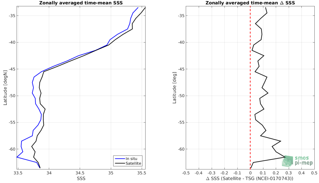
Figure 8: Left panel: Zonal mean SSS from SMAP SSS L4 OI v1 - 7 Days (IPRC) satellite product (black) and from TSG (NCEI-0170743) (blue). Right panel: Zonal mean of \Delta SSS (Satellite - TSG (NCEI-0170743)) for all the collected Pi-MEP match-up pairs estimated over the full satellite product period.
