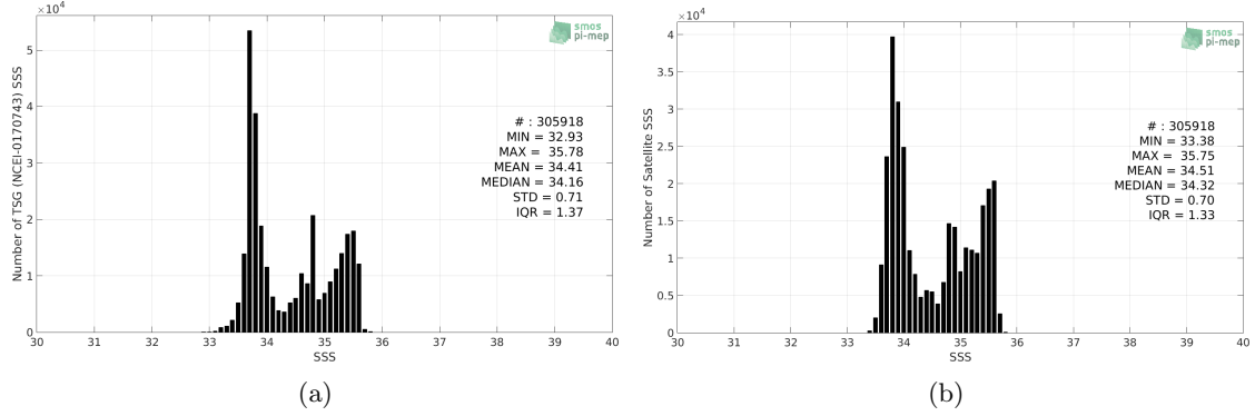
Figure 2: Histograms of SSS from TSG (NCEI-0170743) (a) and SMAP SSS L4 OI v1 - 7 Days (IPRC) (b) considering all match-up pairs per bins of 0.1 over the Global Ocean Pi-MEP region and for the full satellite product period.
