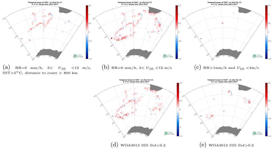
Figure 12: Temporal mean gridded over spatial boxes of size 1^\circ \times 1^\circ of \Delta SSS (SMAP SSS L4 OI v1 - 7day (IPRC) - TSG (NCEI-0170743)) for 5 different subdatasets corresponding to: RR=0 mm/h, 3 < U_{10} < 12 m/s, SST >5^\circ\text{C} , distance to coast > 800 km (a), RR=0 mm/h, 3 < U_{10} < 12 m/s (b), RR >1 mm/h and U_{10} < 4 m/s (c), WOA2013 SSS Std <0.2 (d), WOA2013 SSS Std >0.2 (e).
