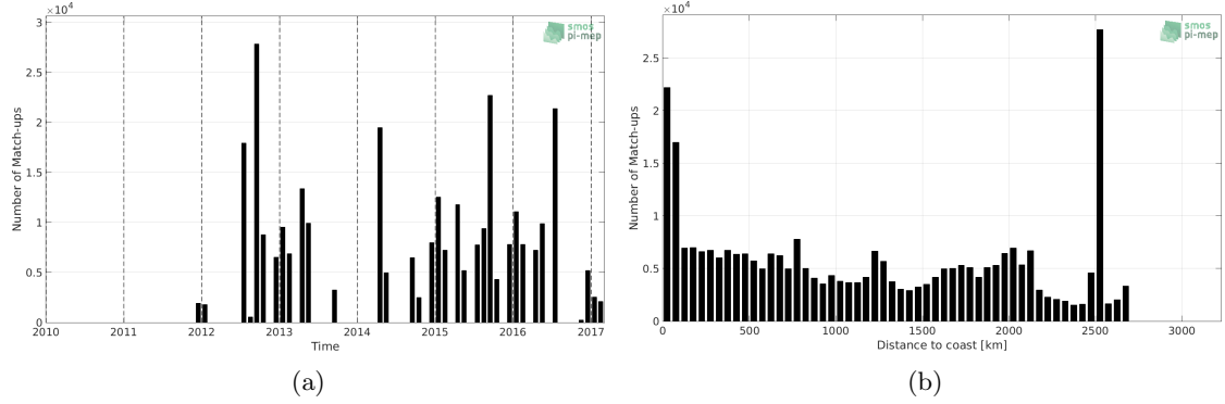
Figure 1: Number of match-ups between TSG (NCEI-0170743) and SMAP SSS L4 OI v1 - 7day (IPRC) SSS as a function of time (a) and as function of the distance to coast (b) over the Global Ocean Pi-MEP region and for the full satellite product period.
