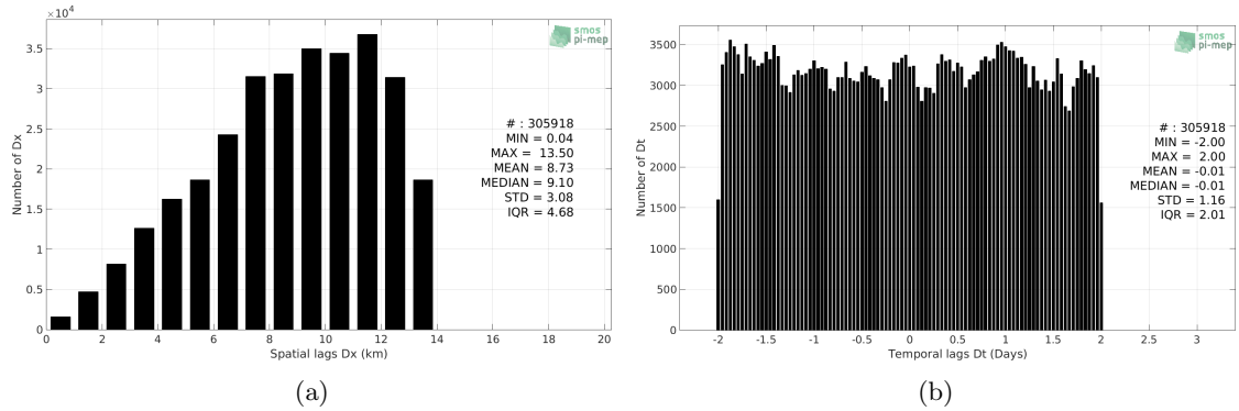
Figure 5: Histograms of the spatial (a) and temporal (b) lags between the location/time of the TSG (NCEI-0170743) measurement and the date of the corresponding SMAP SSS L4 OI v1 - 7day (IPRC) SSS pixel.
