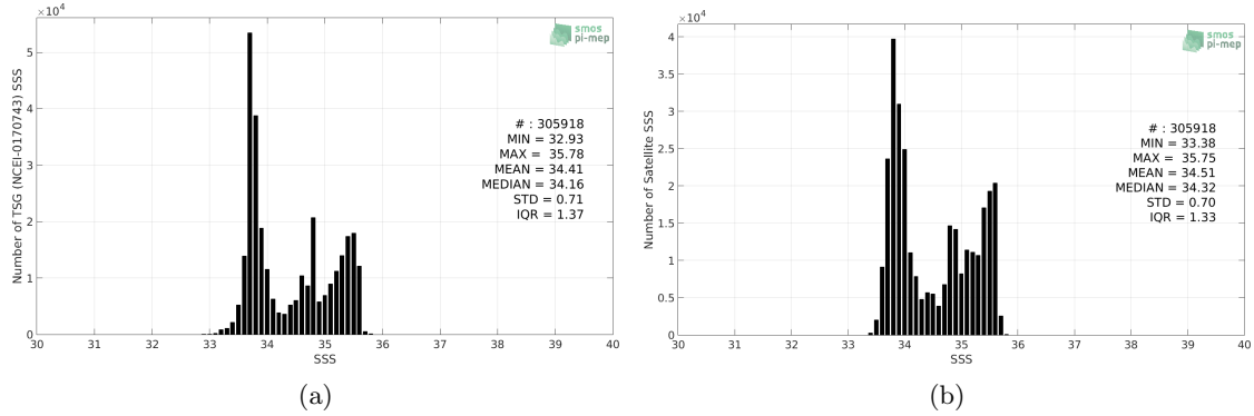
Figure 2: Histograms of SSS from TSG (NCEI-0170743) (a) and SMAP SSS L4 OI v1 - 7day (IPRC) (b) considering all match-up pairs per bins of 0.1 over the Global Ocean Pi-MEP region and for the full satellite product period.
