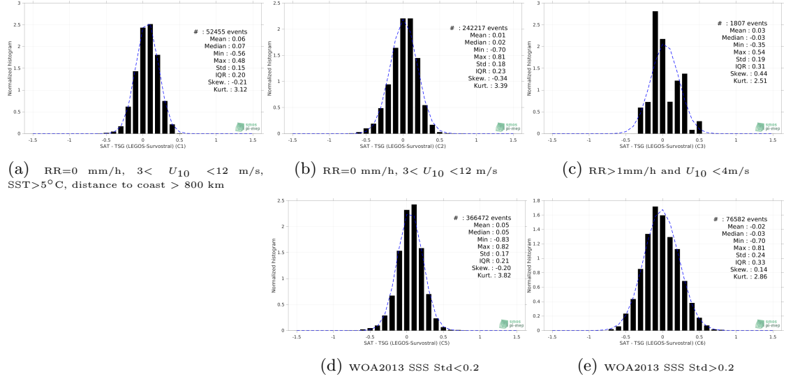
Figure 13: Normalized histogram of \Delta SSS (SMAP SSS L4 OI v1 - 7 Days (IPRC) - TSG (LEGOS-Survostral)) for 5 different subdatasets corresponding to: RR=0 mm/h, 3 < U_{10} < 12 m/s, SST>5°C, distance to coast > 800 km (a), RR=0 mm/h, 3 < U_{10} < 12 m/s (b), RR>1mm/h and U_{10} < 4 m/s (c), WOA2013 SSS Std<0.2 (d), WOA2013 SSS Std>0.2 (e).
