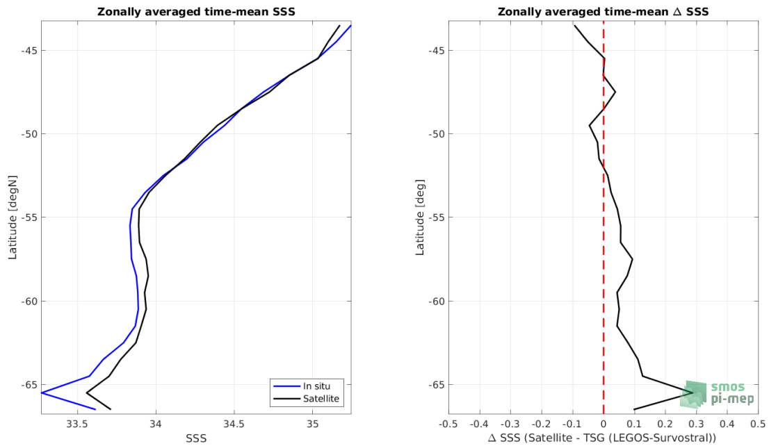
Figure 8: Left panel: Zonal mean SSS from SMAP SSS L4 OI v1 - 7 Days (IPRC) satellite product (black) and from TSG (LEGOS-Survostral) (blue). Right panel: Zonal mean of \Delta SSS (Satellite - TSG (LEGOS-Survostral)) for all the collected Pi-MEP match-up pairs estimated over the full satellite product period.
