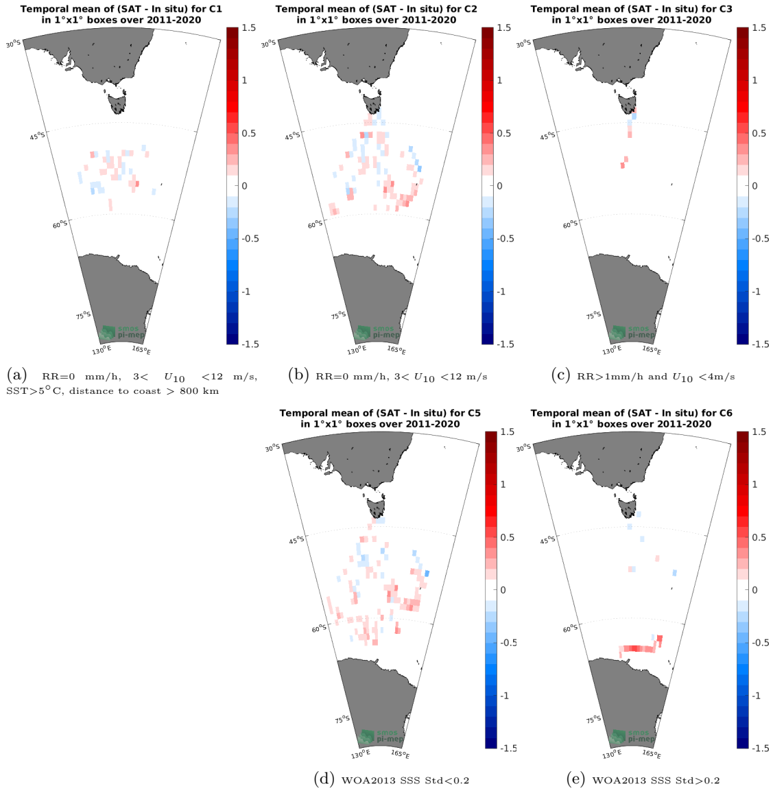
Figure 12: Temporal mean gridded over spatial boxes of size 1^\circ \times 1^\circ of \Delta SSS (SMAP SSS L4 OI v1 - 7 Days (IPRC) - TSG (LEGOS-Survostral)) for 5 different subdatasets corresponding to:RR=0 mm/h, 3 < U_{10} < 12 m/s, SST>5°C, distance to coast > 800 km (a), RR=0 mm/h, 3 < U_{10} < 12 m/s (b), RR>1mm/h and U_{10} < 4 m/s (c), WOA2013 SSS Std<0.2 (d), WOA2013 SSS Std>0.2 (e).
