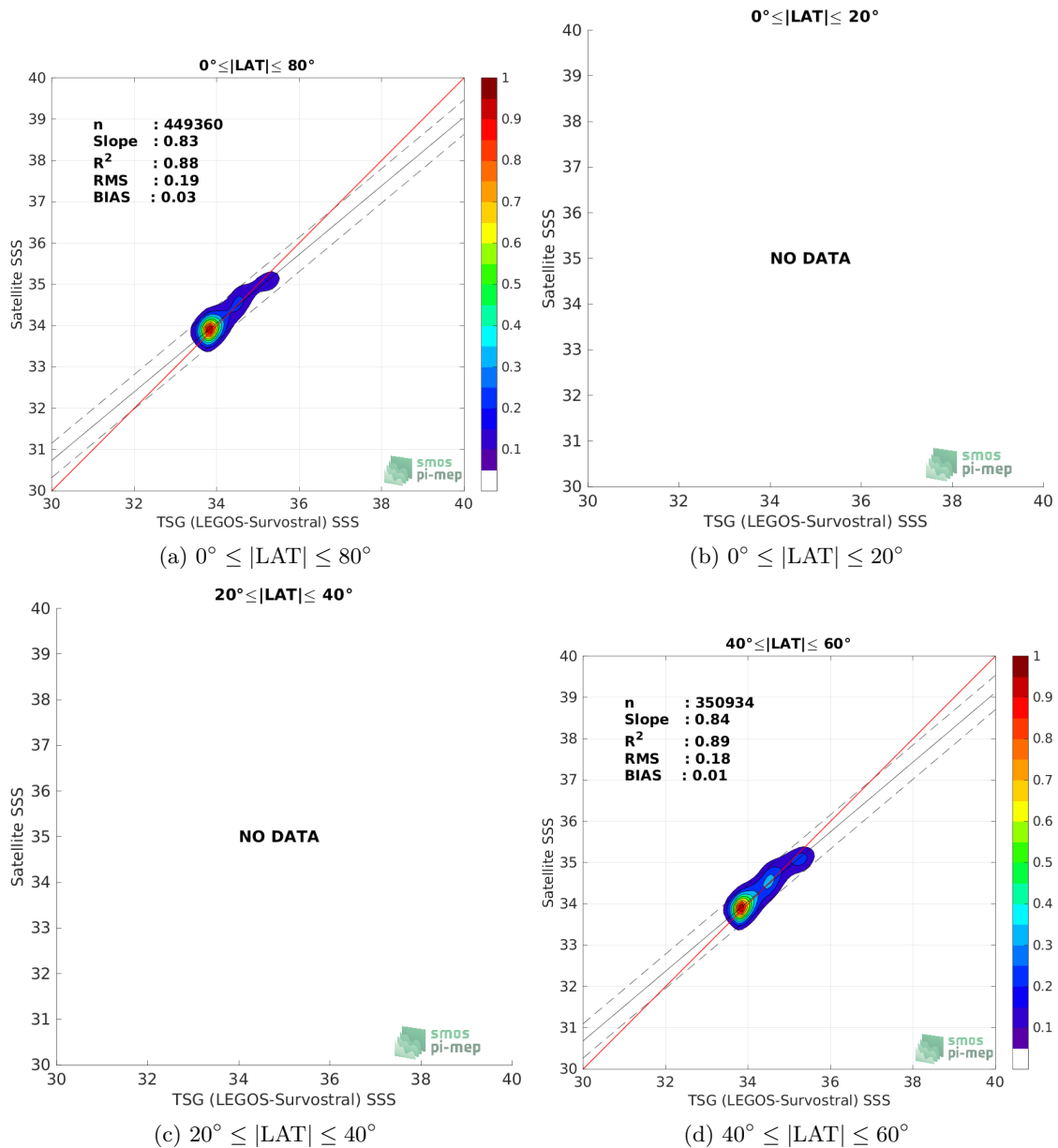
Figure 9: Contour maps of the concentration of SMAP SSS L4 OI v1 - 7 Days (IPRC) SSS (y-axis) versus TSG (LEGOS-Survostral) SSS (x-axis) at match-up pairs for different latitude bands. For each plot, the red line shows x=y . The black thin and dashed lines indicate a linear fit through the data cloud and the \pm 95\% confidence levels, respectively. The number match-up pairs n , the slope and R^2 coefficient of the linear fit, the root mean square (RMS) and the mean bias between satellite and in situ data are indicated for each latitude band in each plot.
