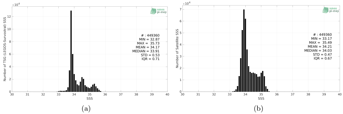
Figure 2: Histograms of SSS from TSG (LEGOS-Survostral) (a) and SMAP SSS L4 OI v1 - 7 Days (IPRC) (b) considering all match-up pairs per bins of 0.1 over the Global Ocean Pi-MEP region and for the full satellite product period.
