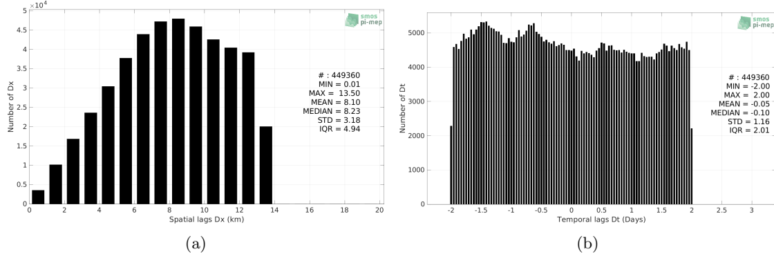
Figure 5: Histograms of the spatial (a) and temporal (b) lags between the location/time of the TSG (LEGOS-Survostral) measurement and the date of the corresponding SMAP SSS L4 OI v1 - 7 Days (IPRC) SSS pixel.
