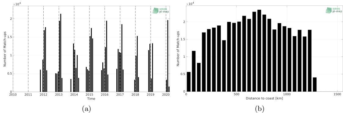
Figure 1: Number of match-ups between TSG (LEGOS-Survostral) and SMAP SSS L4 OI v1 - 7 Days (IPRC) SSS as a function of time (a) and as function of the distance to coast (b) over the Global Ocean Pi-MEP region and for the full satellite product period.
