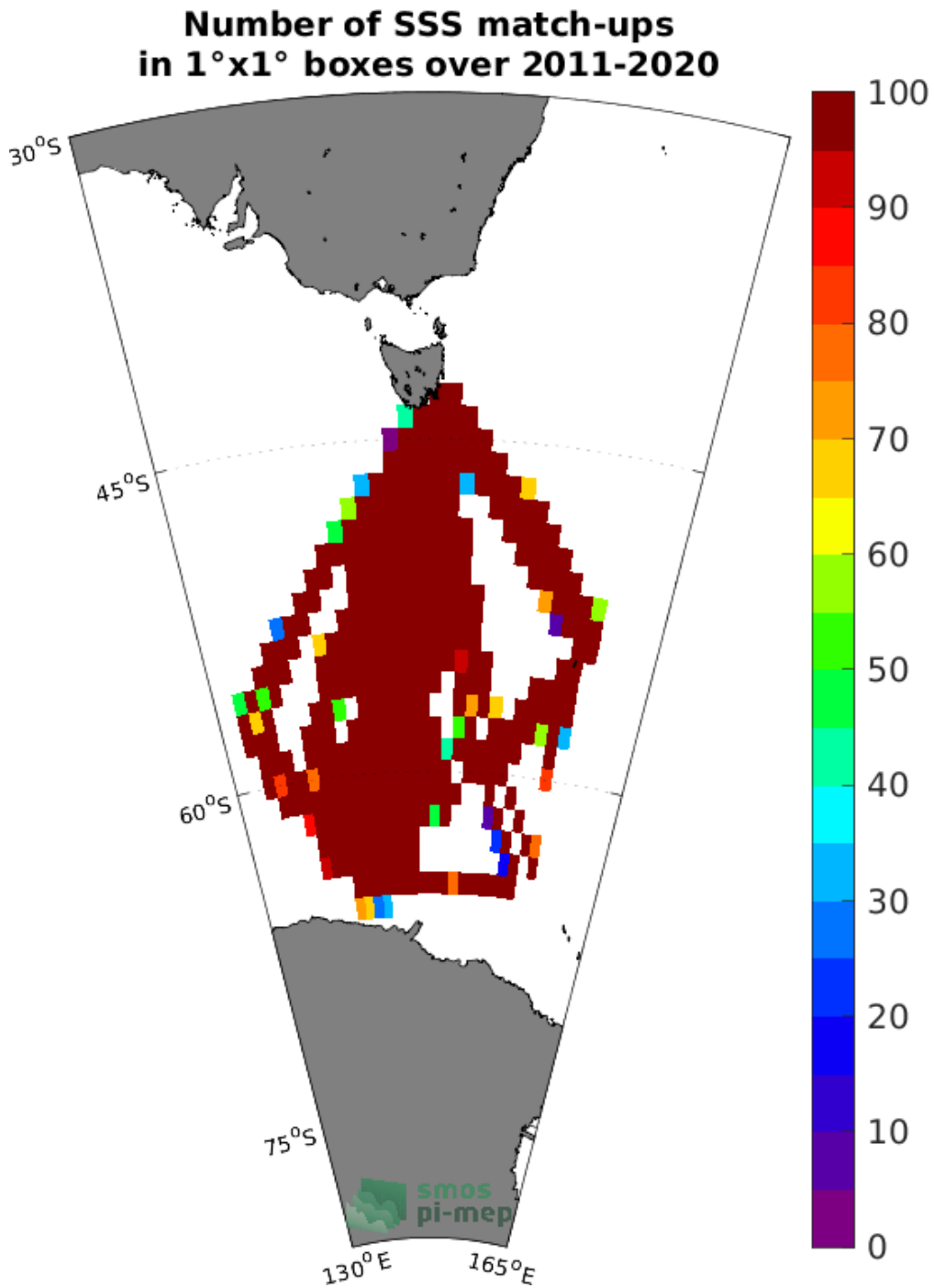
Figure 4: Number of SSS match-ups between TSG (LEGOS-Survostral) SSS and the SMAP SSS L4 OI v1 - 7 Days (IPRC) SSS product for the Global Ocean Pi-MEP region over 1°x1° boxes and for the full satellite product period.
