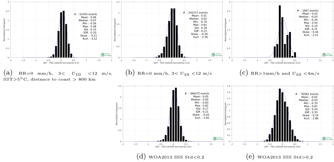
Figure 13: Normalized histogram of \Delta SSS (SMAP SSS L4 OI v1 - 7 Days (IPRC) - TSG (LEGOS-Survostral)) for 5 different subdatasets corresponding to: RR=0 mm/h, 3 < U_{10} < 12 m/s, SST>5°C, distance to coast > 800 km (a), RR=0 mm/h, 3 < U_{10} < 12 m/s (b), RR>1mm/h and U_{10} < 4 m/s (c), WOA2013 SSS Std<0.2 (d), WOA2013 SSS Std>0.2 (e).
