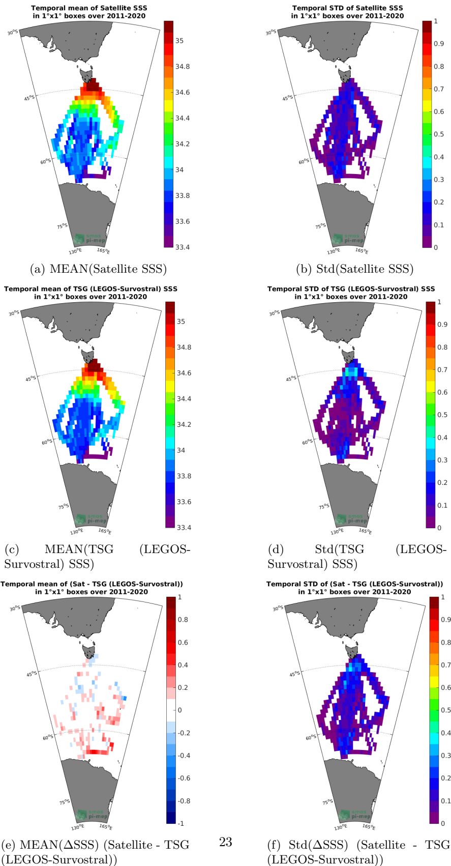
Figure 6: Temporal mean (left) and Std (right) of SSS from SMAP SSS L4 OI v1 - 7 Days (IPRC) (top), TSG (LEGOS-Survostral) (middle), and of \Delta SSS (Satellite - TSG (LEGOS-Survostral)). Only match-up pairs are used to generate these maps.
