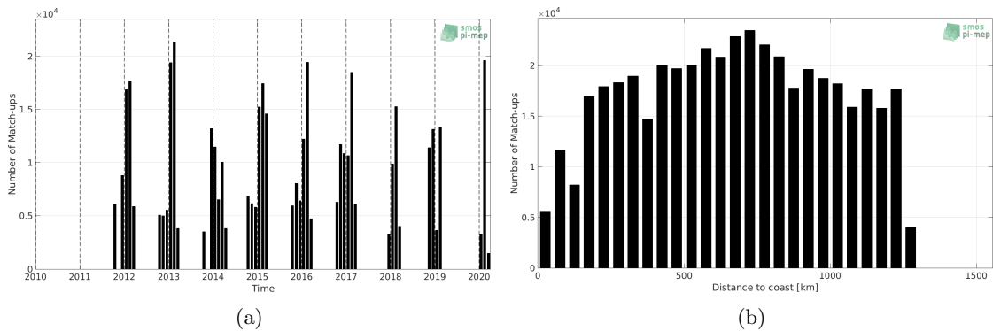
Figure 1: Number of match-ups between TSG (LEGOS-Survostral) and SMAP SSS L4 OI v1 - 7day (IPRC) SSS as a function of time (a) and as function of the distance to coast (b) over the Global Ocean Pi-MEP region and for the full satellite product period.
