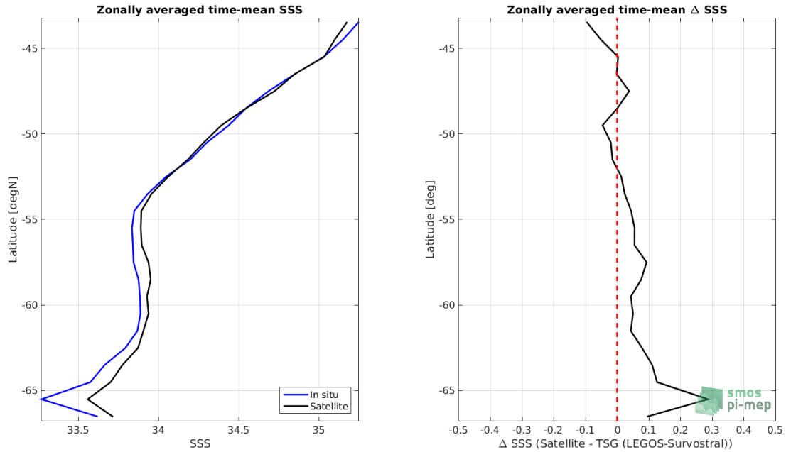
Figure 8: Left panel: Zonal mean SSS from SMAP SSS L4 OI v1 - 7day (IPRC) satellite product (black) and from TSG (LEGOS-Survostral) (blue). Right panel: Zonal mean of \Delta SSS (Satellite - TSG (LEGOS-Survostral)) for all the collected Pi-MEP match-up pairs estimated over the full satellite product period.
