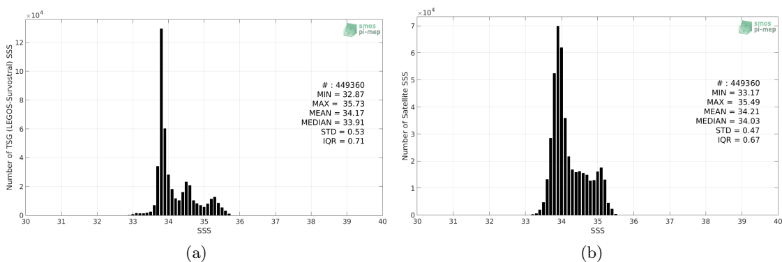
Figure 2: Histograms of SSS from TSG (LEGOS-Survostral) (a) and SMAP SSS L4 OI v1 - 7day (IPRC) (b) considering all match-up pairs per bins of 0.1 over the Global Ocean Pi-MEP region and for the full satellite product period.
