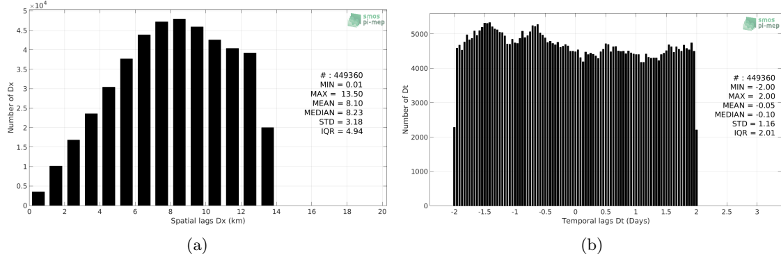
Figure 5: Histograms of the spatial (a) and temporal (b) lags between the location/time of the TSG (LEGOS-Survostral) measurement and the date of the corresponding SMAP SSS L4 OI v1 - 7day (IPRC) SSS pixel.
