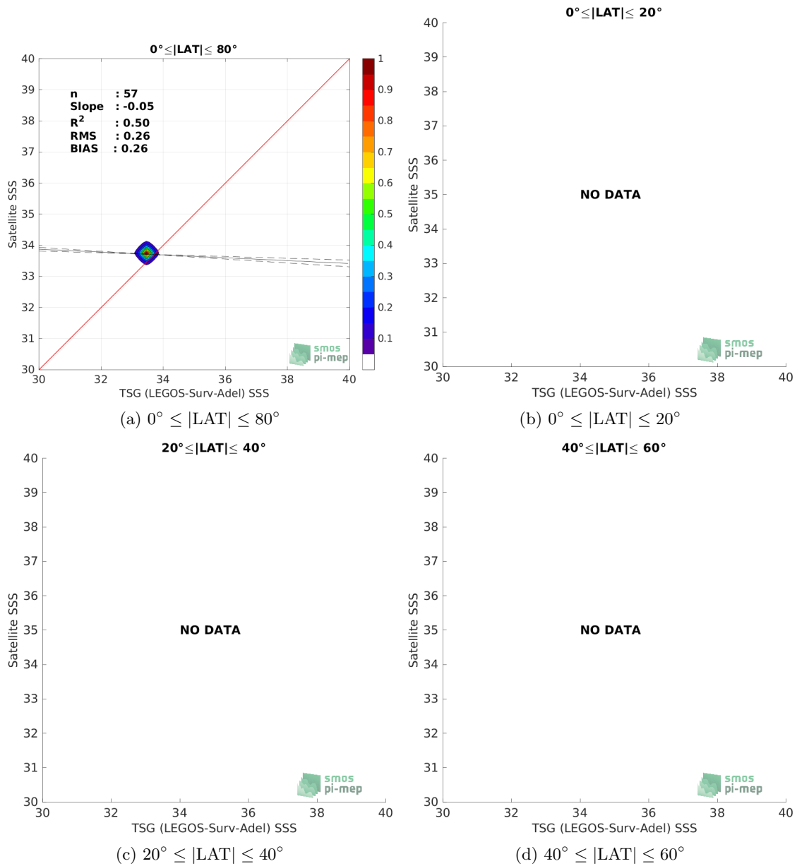
Figure 9: Contour maps of the concentration of SMAP SSS L4 OI v1 - 7 Days (IPRC) SSS (y-axis) versus TSG (LEGOS-Surv-Adel) SSS (x-axis) at match-up pairs for different latitude bands. For each plot, the red line shows x=y . The black thin and dashed lines indicate a linear fit through the data cloud and the \pm 95\% confidence levels, respectively. The number match-up pairs n , the slope and R^2 coefficient of the linear fit, the root mean square (RMS) and the mean bias between satellite and in situ data are indicated for each latitude band in each plots.
