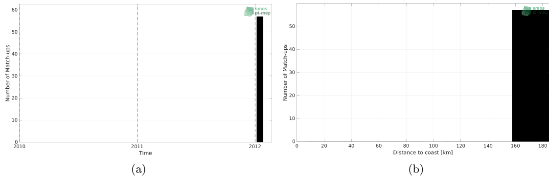
Figure 1: Number of match-ups between TSG (LEGOS-Surv-Adel) and SMAP SSS L4 OI v1 - 7 Days (IPRC) SSS as a function of time (a) and as function of the distance to coast (b) over the Global Ocean Pi-MEP region and for the full satellite product period.
