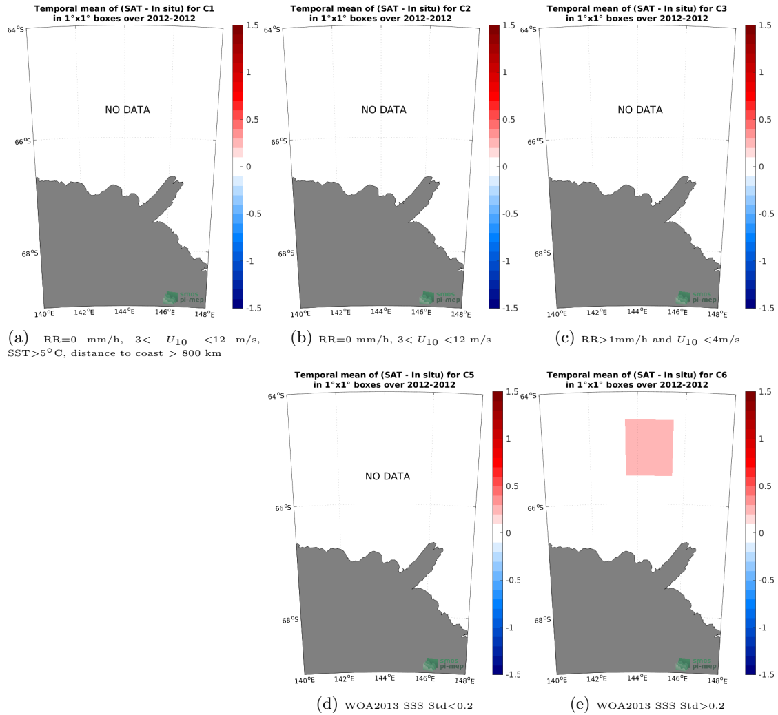
Figure 12: Temporal mean gridded over spatial boxes of size 1^\circ \times 1^\circ of \Delta SSS (SMAP SSS L4 OI v1 - 7 Days (IPRC) - TSG (LEGOS-Surv-Adel)) for 5 different subdatasets corresponding to: RR=0 mm/h, 3 < U_{10} < 12 m/s, SST>5°C, distance to coast > 800 km (a), RR=0 mm/h, 3 < U_{10} < 12 m/s (b), RR>1mm/h and U_{10} < 4 m/s (c), WOA2013 SSS Std<0.2 (d), WOA2013 SSS Std>0.2 (e).
