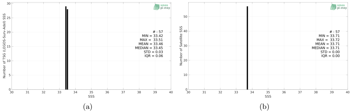
Figure 2: Histograms of SSS from TSG (LEGOS-Surv-Adel) (a) and SMAP SSS L4 OI v1 - 7 Days (IPRC) (b) considering all match-up pairs per bins of 0.1 over the Global Ocean Pi-MEP region and for the full satellite product period.
