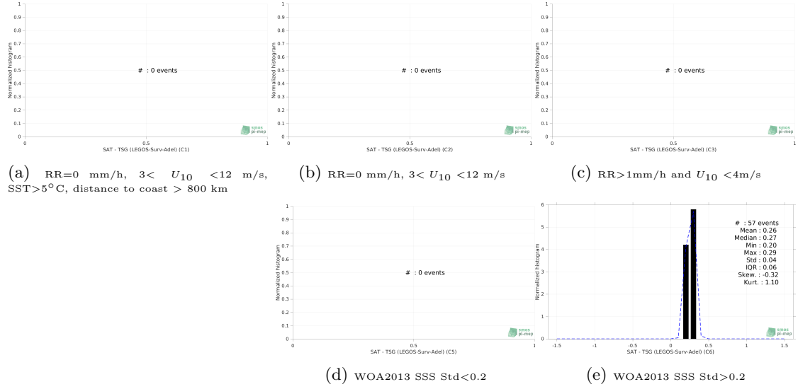
Figure 13: Normalized histogram of \Delta SSS (SMAP SSS L4 OI v1 - 7 Days (IPRC) - TSG (LEGOS-Surv-Adel)) for 5 different subdatasets corresponding to: RR=0 mm/h, 3 < U_{10} < 12 m/s, SST > 5°C, distance to coast > 800 km (a), RR=0 mm/h, 3 < U_{10} < 12 m/s (b), RR > 1mm/h and U_{10} < 4 m/s (c), WOA2013 SSS Std < 0.2 (d), WOA2013 SSS Std > 0.2 (e).
