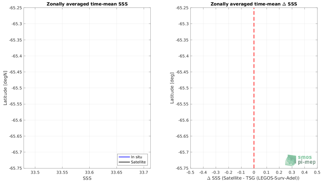
Figure 8: Left panel: Zonal mean SSS from SMAP SSS L4 OI v1 - 7 Days (IPRC) satellite product (black) and from TSG (LEGOS-Surv-Adel) (blue). Right panel: Zonal mean of \Delta SSS (Satellite - TSG (LEGOS-Surv-Adel)) for all the collected Pi-MEP match-up pairs estimated over the full satellite product period.
