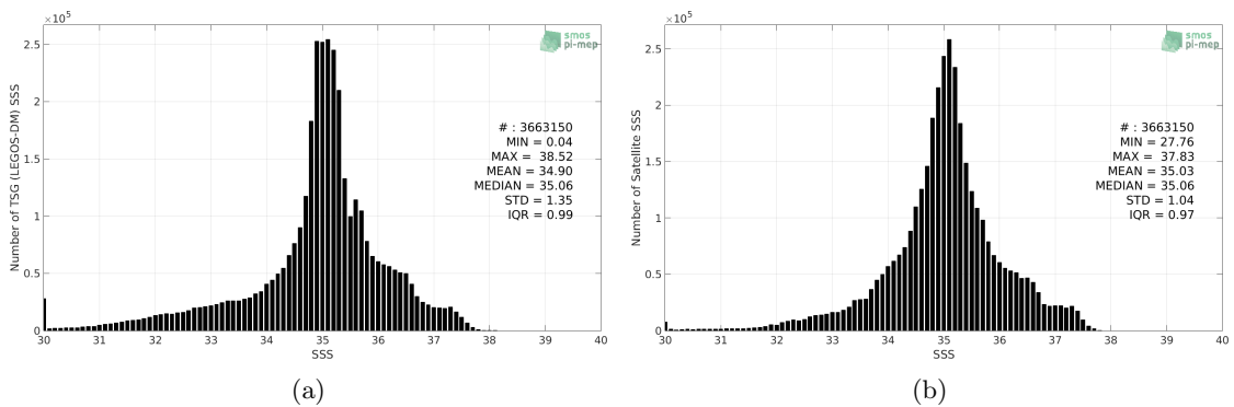
Figure 2: Histograms of SSS from TSG (LEGOS-DM) (a) and SMAP SSS L4 OI v1 - 7day (IPRC) (b) considering all match-up pairs per bins of 0.1 over the Global Ocean Pi-MEP region and for the full satellite product period.
