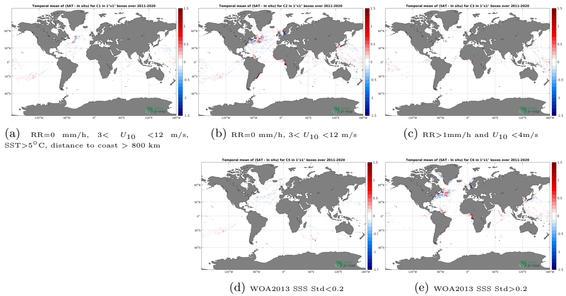
Figure 12: Temporal mean gridded over spatial boxes of size 1^\circ \times 1^\circ of \Delta SSS (SMAP SSS L4 OI v1 - 7day (IPRC) - TSG (LEGOS-DM)) for 5 different subdatasets corresponding to:RR=0 mm/h, 3 < U_{10} < 12 m/s, SST>5°C, distance to coast > 800 km (a), RR=0 mm/h, 3 < U_{10} < 12 m/s (b), RR>1mm/h and U_{10} < 4 m/s (c), WOA2013 SSS Std<0.2 (d), WOA2013 SSS Std>0.2 (e).
