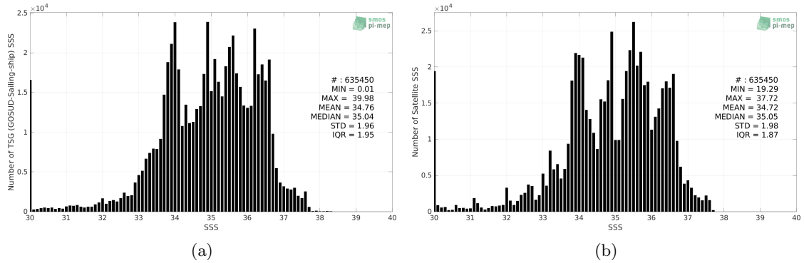
Figure 2: Histograms of SSS from TSG (GOSUD-Sailing-ship) (a) and SMAP SSS L4 OI v1 - 7 Days (IPRC) (b) considering all match-up pairs per bins of 0.1 over the Global Ocean Pi-MEP region and for the full satellite product period.
