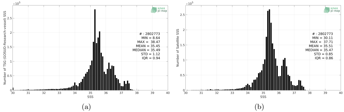
Figure 2: Histograms of SSS from TSG (GOSUD-Research-vessel) (a) and SMAP SSS L4 OI v1 - 7day (IPRC) (b) considering all match-up pairs per bins of 0.1 over the Global Ocean Pi-MEP region and for the full satellite product period.
