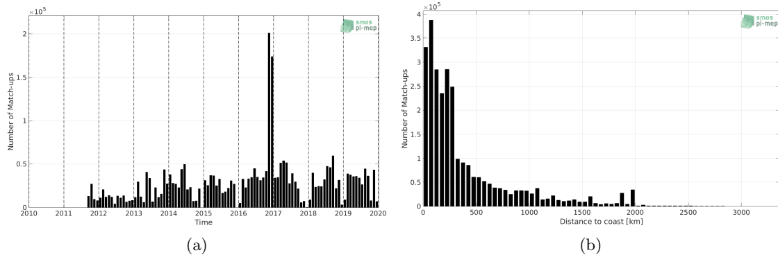
Figure 1: Number of match-ups between TSG (GOSUD-Research-vessel) and SMAP SSS L4 OI v1 - 7day (IPRC) SSS as a function of time (a) and as function of the distance to coast (b) over the Global Ocean Pi-MEP region and for the full satellite product period.
