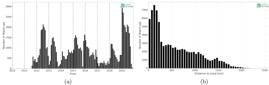
Figure 1: Number of match-ups between Marine mammals and SMAP SSS L4 OI v1 - 7 Days (IPRC) SSS as a function of time (a) and as function of the distance to coast (b) over the Global Ocean Pi-MEP region and for the full satellite product period.
