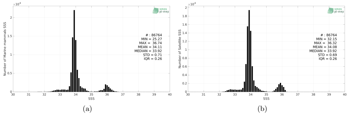
Figure 2: Histograms of SSS from Marine mammals (a) and SMAP SSS L4 OI v1 - 7 Days (IPRC) (b) considering all match-up pairs per bins of 0.1 over the Global Ocean Pi-MEP region and for the full satellite product period.
