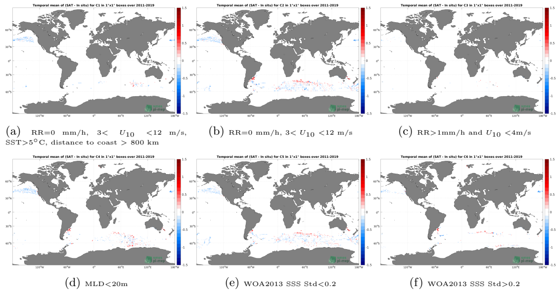
Figure 12: Temporal mean gridded over spatial boxes of size 1^\circ \times 1^\circ of \Delta SSS (SMAP SSS L4 OI v1 - 7 Days (IPRC) - Marine mammals) for 6 different subdatasets corresponding to:RR=0 mm/h, 3 < U_{10} < 12 m/s, SST >5^\circ C, distance to coast > 800 km (a), RR=0 mm/h, 3 < U_{10} < 12 m/s (b), RR >1 mm/h and U_{10} < 4 m/s (c),MLD <20 m (d),WOA2013 SSS Std <0.2 (e),WOA2013 SSS Std >0.2 (f).
