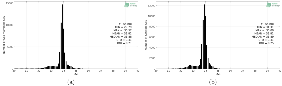
Figure 2: Histograms of SSS from Marine mammals (a) and SMAP SSS L4 OI v1 - 7 Days (IPRC) (b) considering all match-up pairs per bins of 0.1 over the Global Ocean Pi-MEP region and for the full satellite product period.
