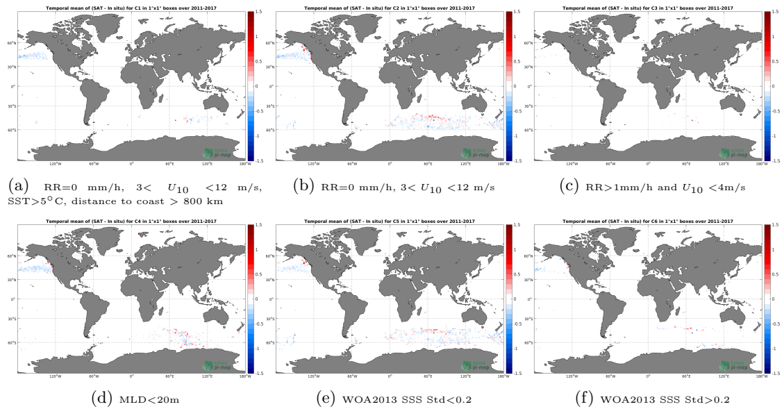
Figure 12: Temporal mean gridded over spatial boxes of size 1°x1° of \Delta SSS (SMAP SSS L4 OI v1 - 7day (IPRC) - Sea mammals) for 6 different subdatasets corresponding to:RR=0 mm/h, 3 < U_{10} < 12 m/s, SST>5°C, distance to coast > 800 km (a), RR=0 mm/h, 3 < U_{10} < 12 m/s (b), RR>1mm/h and U_{10} < 4 m/s (c),MLD<20m (d),WOA2013 SSS Std<0.2 (e),WOA2013 SSS Std>0.2 (f).
