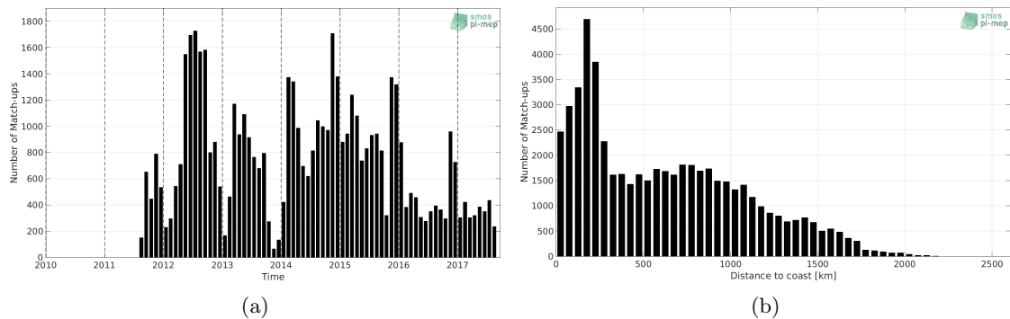
Figure 1: Number of match-ups between Sea mammals and SMAP SSS L4 OI v1 - 7day (IPRC) SSS as a function of time (a) and as function of the distance to coast (b) over the Global Ocean Pi-MEP region and for the full satellite product period.
