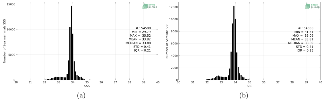
Figure 2: Histograms of SSS from Sea mammals (a) and SMAP SSS L4 OI v1 - 7day (IPRC) (b) considering all match-up pairs per bins of 0.1 over the Global Ocean Pi-MEP region and for the full satellite product period.
