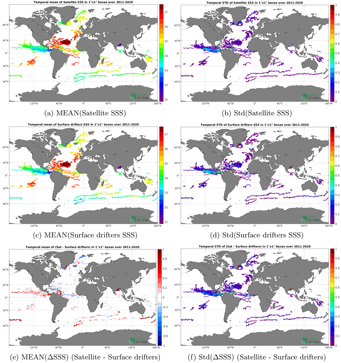
Figure 5: Temporal mean (left) and Std (right) of SSS from SMAP SSS L4 OI v1 - 7day (IPRC) (top), Surface drifters (middle), and of \Delta SSS (Satellite - Surface drifters). Only match-up pairs are used to generate these maps.
