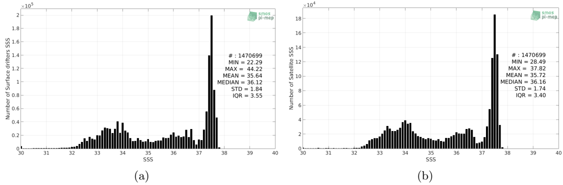
Figure 2: Histograms of SSS from Surface drifters (a) and SMAP SSS L4 OI v1 - 7day (IPRC) (b) considering all match-up pairs per bins of 0.1 over the Global Ocean Pi-MEP region and for the full satellite product period.
