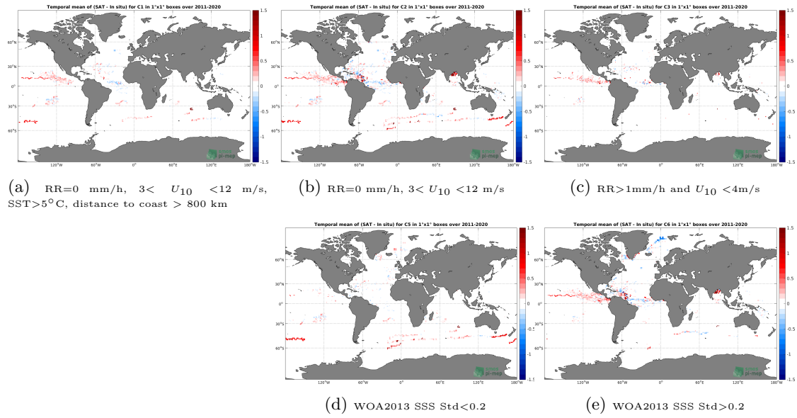
Figure 11: Temporal mean gridded over spatial boxes of size 1^\circ \times 1^\circ of \Delta SSS (SMAP SSS L4 OI v1 - 7day (IPRC) - Surface drifters) for 5 different subdatasets corresponding to: RR=0 mm/h, 3 < U_{10} < 12 m/s, SST > 5^\circ C , distance to coast > 800 km (a), RR=0 mm/h, 3 < U_{10} < 12 m/s (b), RR > 1 mm/h and U_{10} < 4 m/s (c), WOA2013 SSS Std < 0.2 (d), WOA2013 SSS Std > 0.2 (e).
