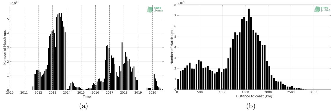
Figure 1: Number of match-ups between Surface drifters and SMAP SSS L4 OI v1 - 7day (IPRC) SSS as a function of time (a) and as function of the distance to coast (b) over the Global Ocean Pi-MEP region and for the full satellite product period.
