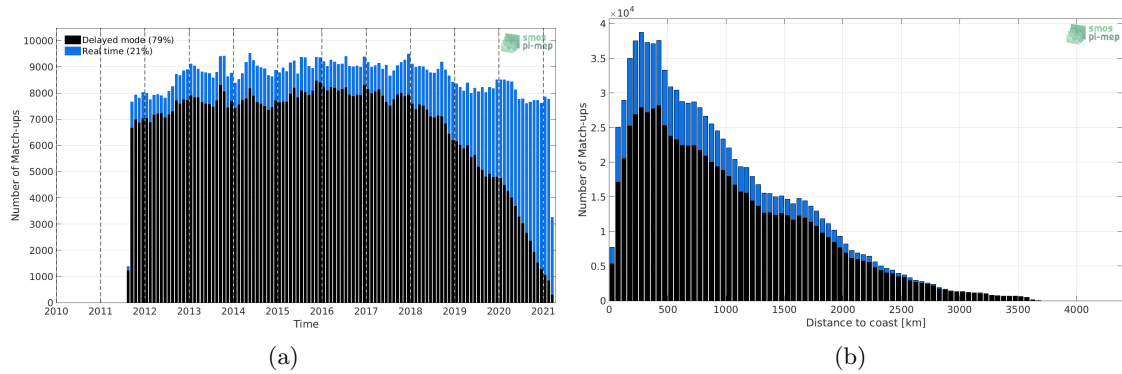
Figure 1: Number of match-ups between Argo and SMAP SSS L4 OI v1 - 7 Days (IPRC) SSS as a function of time (a) and as function of the distance to coast (b) over the Global Ocean Pi-MEP region and for the full satellite product period.
