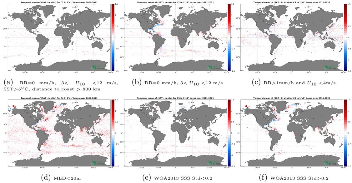
Figure 12: Temporal mean gridded over spatial boxes of size 1^\circ \times 1^\circ of \Delta SSS (SMAP SSS L4 OI v1 - 7 Days (IPRC) - Argo) for 6 different subdatasets corresponding to: RR=0 mm/h, 3 < U_{10} < 12 m/s, SST > 5^\circ\text{C} , distance to coast > 800 km (a), RR=0 mm/h, 3 < U_{10} < 12 m/s (b), RR > 1 mm/h and U_{10} < 4 m/s (c), MLD < 20 m (d), WOA2013 SSS Std < 0.2 (e), WOA2013 SSS Std > 0.2 (f).
