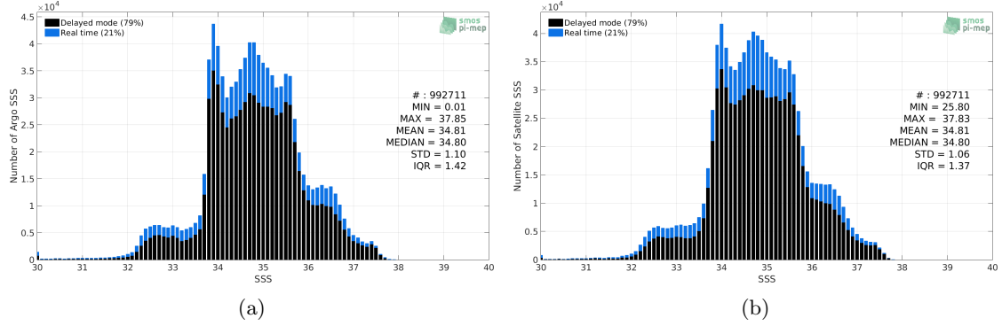
Figure 2: Histograms of SSS from Argo (a) and SMAP SSS L4 OI v1 - 7 Days (IPRC) (b) considering all match-up pairs per bins of 0.1 over the Global Ocean Pi-MEP region and for the full satellite product period.
