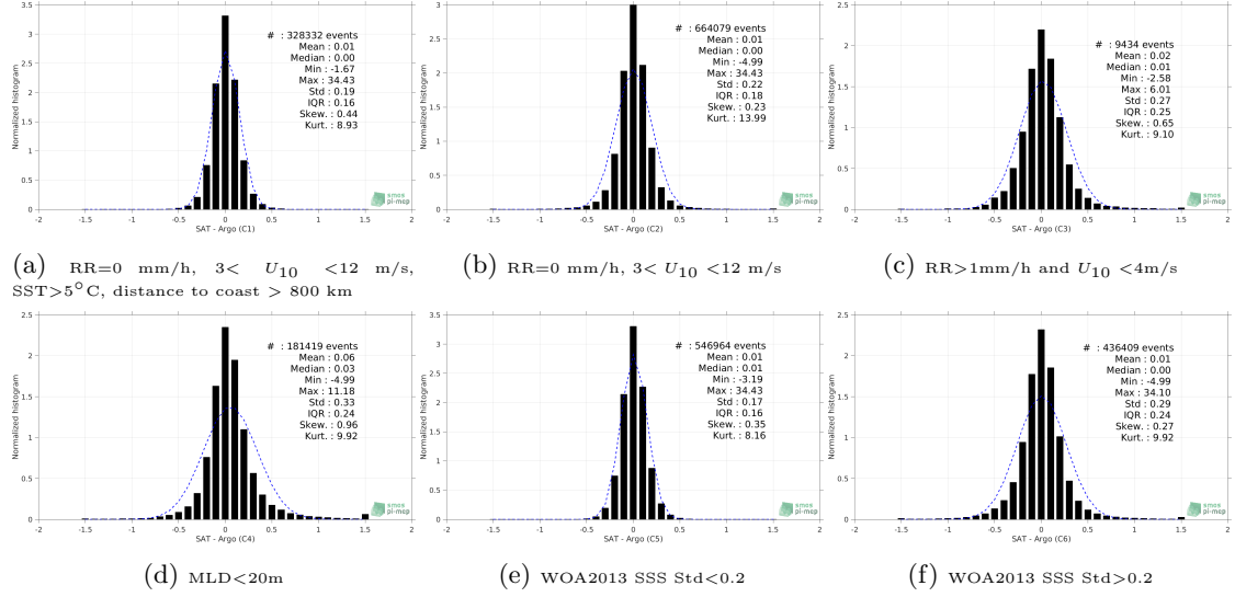
Figure 13: Normalized histogram of \Delta\text{SSS} (SMAP SSS L4 OI v1 - 7 Days (IPRC) - Argo) for 6 different subdatasets corresponding to: RR=0 mm/h, 3 < U_{10} < 12 m/s, SST>5°C, distance to coast > 800 km (a), RR=0 mm/h, 3 < U_{10} < 12 m/s (b), RR>1mm/h and U_{10} < 4 m/s (c), MLD<20m (d), WOA2013 SSS Std<0.2 (e), WOA2013 SSS Std>0.2 (f).
