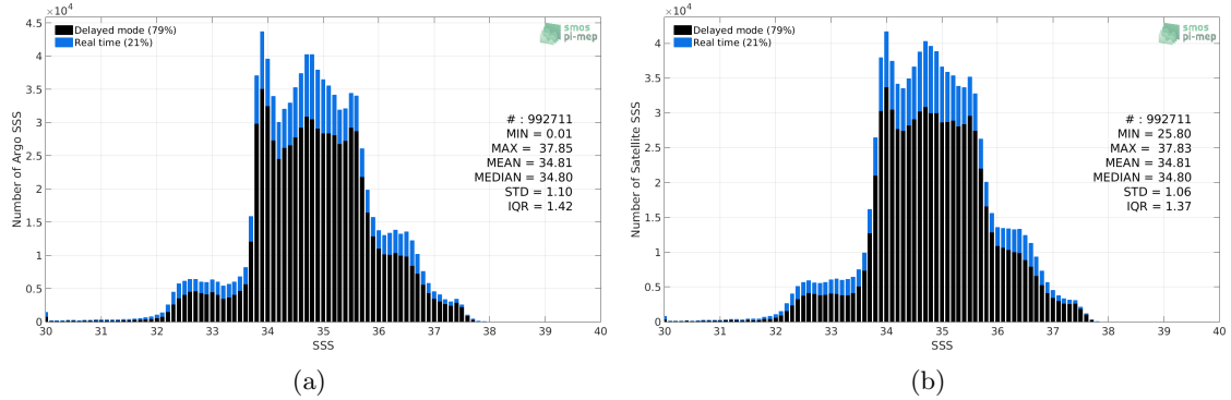
Figure 2: Histograms of SSS from Argo (a) and SMAP SSS L4 OI v1 - 7day (IPRC) (b) considering all match-up pairs per bins of 0.1 over the Global Ocean Pi-MEP region and for the full satellite product period.
