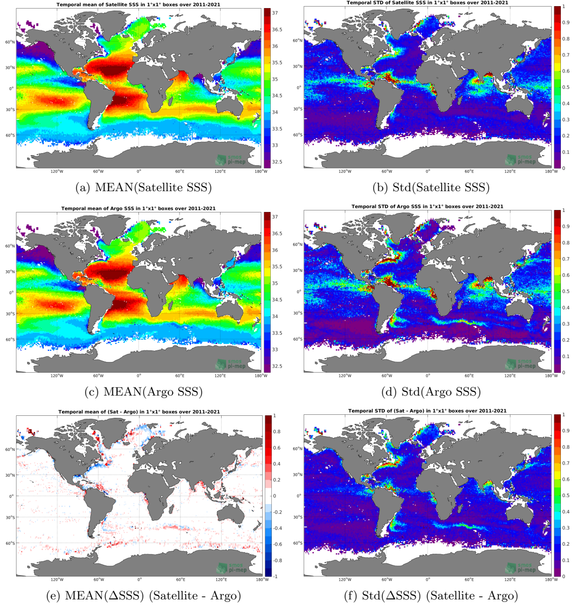
Figure 6: Temporal mean (left) and Std (right) of SSS from SMAP SSS L4 OI v1 - 7day (IPRC) (top), Argo (middle), and of \Delta SSS (Satellite - Argo). Only match-up pairs are used to generate these maps.
