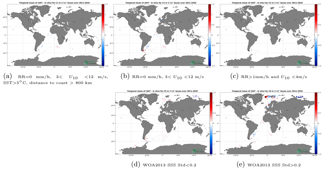
Figure 12: Temporal mean gridded over spatial boxes of size 1^\circ \times 1^\circ of \Delta SSS (SMAP SSS L4 OI v1 - Monthly (IPRC) - TSG (Polarstern)) for 5 different subdatasets corresponding to: RR=0 mm/h, 3 < U_{10} < 12 m/s, SST > 5^\circ C , distance to coast > 800 km (a), RR=0 mm/h, 3 < U_{10} < 12 m/s (b), RR > 1 mm/h and U_{10} < 4 m/s (c), WOA2013 SSS Std < 0.2 (d), WOA2013 SSS Std > 0.2 (e).
