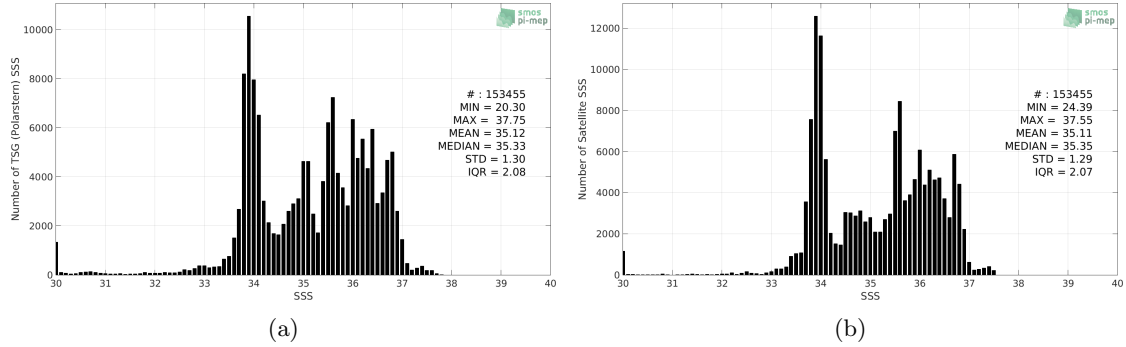
Figure 2: Histograms of SSS from TSG (Polarstern) (a) and SMAP SSS L4 OI v1 - Monthly (IPRC) (b) considering all match-up pairs per bins of 0.1 over the Global Ocean Pi-MEP region and for the full satellite product period.
