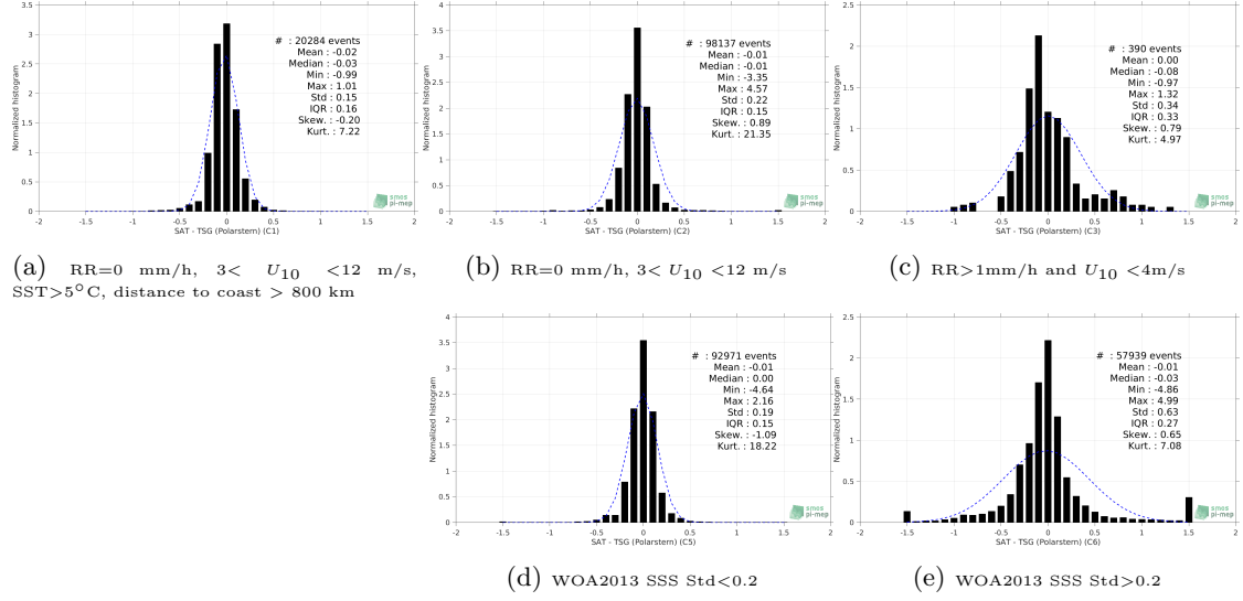
Figure 13: Normalized histogram of \Delta\text{SSS} (SMAP SSS L4 OI v1 - Monthly (IPRC) - TSG (Polarstern)) for 5 different subdatasets corresponding to: RR=0 mm/h, 3 < U_{10} < 12 m/s, SST>5°C, distance to coast > 800 km (a), RR=0 mm/h, 3 < U_{10} < 12 m/s (b), RR>1mm/h and U_{10} < 4 m/s (c), WOA2013 SSS Std<0.2 (d), WOA2013 SSS Std>0.2 (e).
