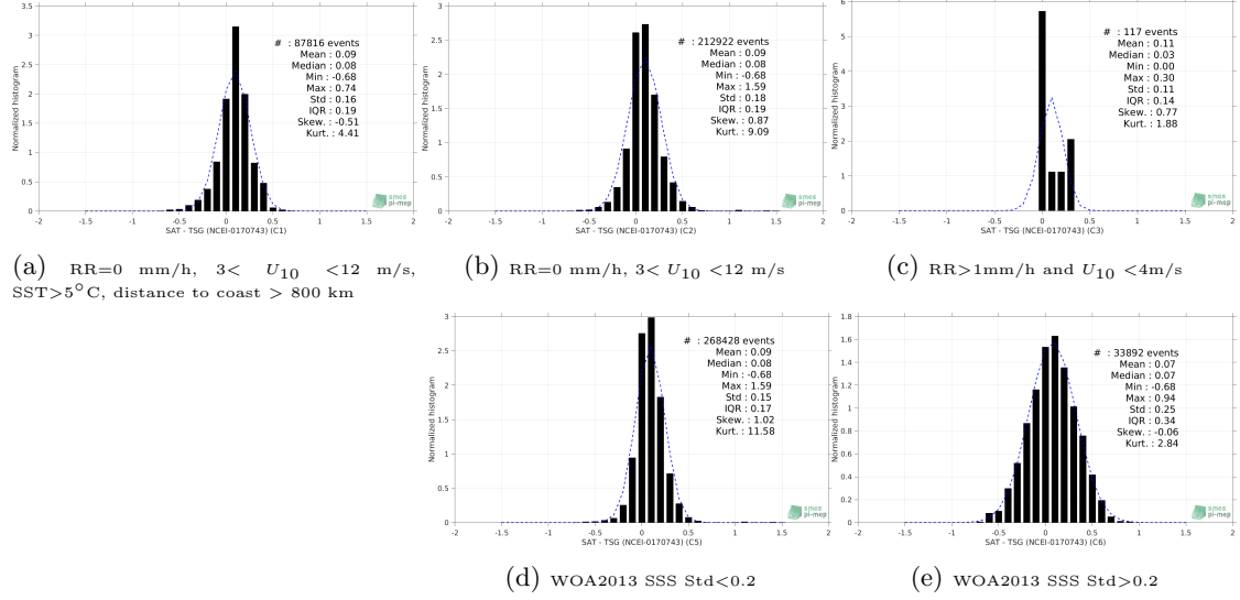
Figure 13: Normalized histogram of \Delta\text{SSS} (SMAP SSS L4 OI v1 - Monthly (IPRC) - TSG (NCEI-0170743)) for 5 different subdatasets corresponding to: RR=0 mm/h, 3 < U_{10} < 12 m/s, SST > 5^\circ\text{C} , distance to coast > 800 km (a), RR=0 mm/h, 3 < U_{10} < 12 m/s (b), RR > 1 mm/h and U_{10} < 4 m/s (c), WOA2013 SSS Std < 0.2 (d), WOA2013 SSS Std > 0.2 (e).
