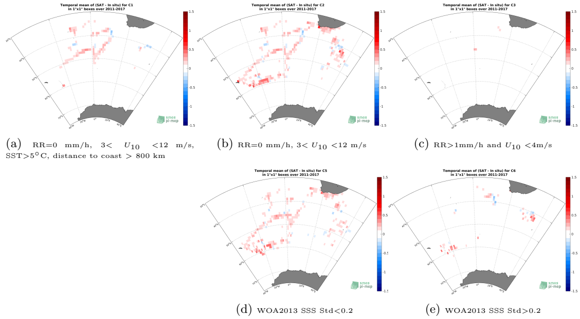
Figure 12: Temporal mean gridded over spatial boxes of size 1^\circ \times 1^\circ of \Delta SSS (SMAP SSS L4 OI v1 - Monthly (IPRC) - TSG (NCEI-0170743)) for 5 different subdatasets corresponding to: RR=0 mm/h, 3 < U_{10} < 12 m/s, SST >5^\circ\text{C} , distance to coast > 800 km (a), RR=0 mm/h, 3 < U_{10} < 12 m/s (b), RR >1 mm/h and U_{10} < 4 m/s (c), WOA2013 SSS Std <0.2 (d), WOA2013 SSS Std >0.2 (e).
