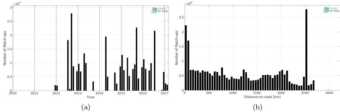
Figure 1: Number of match-ups between TSG (NCEI-0170743) and SMAP SSS L4 OI v1 - Monthly (IPRC) SSS as a function of time (a) and as function of the distance to coast (b) over the Global Ocean Pi-MEP region and for the full satellite product period.
