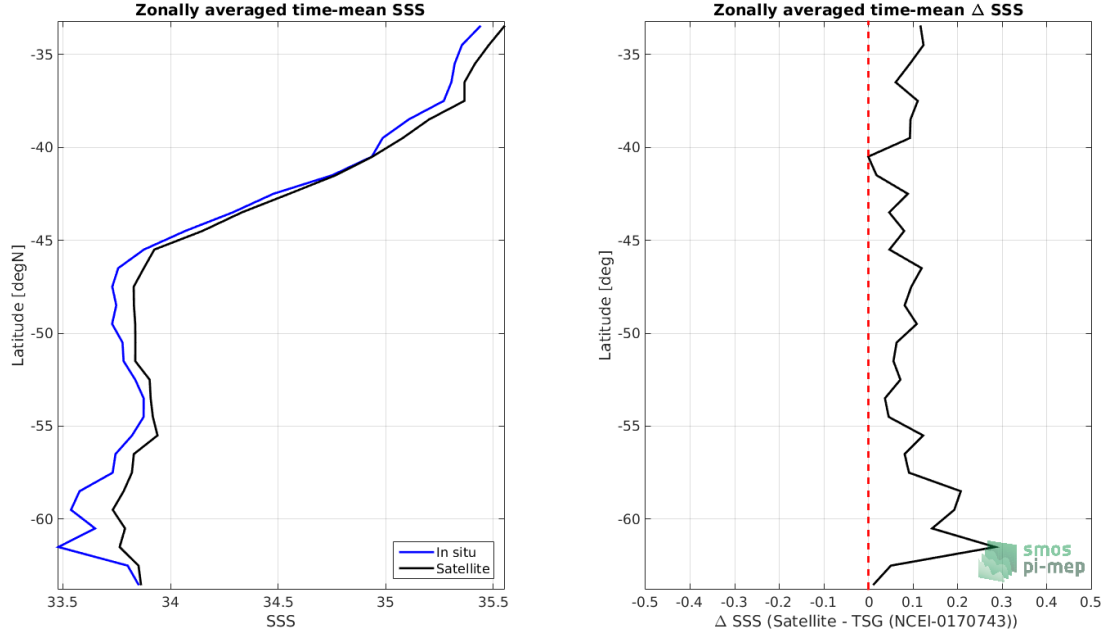
Figure 8: Left panel: Zonal mean SSS from SMAP SSS L4 OI v1 - Monthly (IPRC) satellite product (black) and from TSG (NCEI-0170743) (blue). Right panel: Zonal mean of \Delta SSS (Satellite - TSG (NCEI-0170743)) for all the collected Pi-MEP match-up pairs estimated over the full satellite product period.
