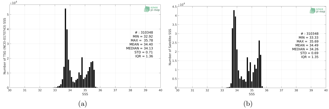
Figure 2: Histograms of SSS from TSG (NCEI-0170743) (a) and SMAP SSS L4 OI v1 - Monthly (IPRC) (b) considering all match-up pairs per bins of 0.1 over the Global Ocean Pi-MEP region and for the full satellite product period.
