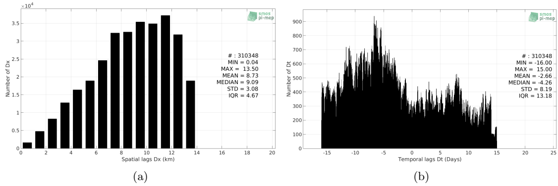
Figure 5: Histograms of the spatial (a) and temporal (b) lags between the location/time of the TSG (NCEI-0170743) measurement and the date of the corresponding SMAP SSS L4 OI v1 - Monthly (IPRC) SSS pixel.
