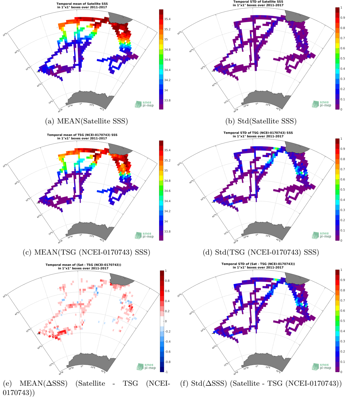
Figure 6: Temporal mean (left) and Std (right) of SSS from SMAP SSS L4 OI v1 - Monthly (IPRC) (top), TSG (NCEI-0170743) (middle), and of \Delta SSS (Satellite - TSG (NCEI-0170743)). Only match-up pairs are used to generate these maps.
