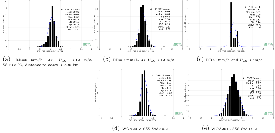
Figure 13: Normalized histogram of \Delta SSS (SMAP SSS L4 OI v1 - Monthly (IPRC) - TSG (NCEI-0170743)) for 5 different subdatasets corresponding to: RR=0 mm/h, 3 < U_{10} < 12 m/s, SST>5°C, distance to coast > 800 km (a), RR=0 mm/h, 3 < U_{10} < 12 m/s (b), RR>1 mm/h and U_{10} < 4 m/s (c), WOA2013 SSS Std<0.2 (d), WOA2013 SSS Std>0.2 (e).
