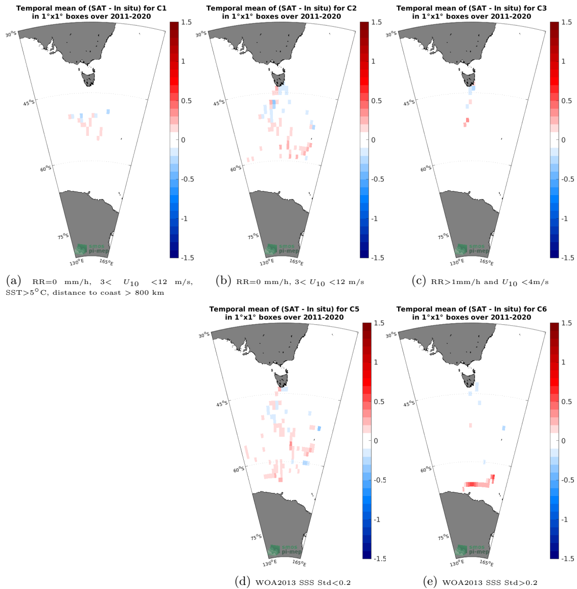
Figure 12: Temporal mean gridded over spatial boxes of size 1^\circ \times 1^\circ of \Delta SSS (SMAP SSS L4 OI v1 - Monthly (IPRC) - TSG (LEGOS-Survostral)) for 5 different subdatasets corresponding to: RR=0 mm/h, 3 < U_{10} < 12 m/s, SST>5°C, distance to coast > 800 km (a), RR=0 mm/h, 3 < U_{10} < 12 m/s (b), RR>1mm/h and U_{10} < 4 m/s (c), WOA2013 SSS Std<0.2 (d), WOA2013 SSS Std>0.2 (e).
