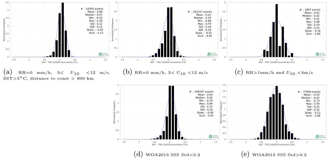
Figure 13: Normalized histogram of \Delta SSS (SMAP SSS L4 OI v1 - Monthly (IPRC) - TSG (LEGOS-Survostral)) for 5 different subdatasets corresponding to: RR=0 mm/h, 3 < U_{10} < 12 m/s, SST>5°C, distance to coast > 800 km (a), RR=0 mm/h, 3 < U_{10} < 12 m/s (b), RR>1mm/h and U_{10} < 4 m/s (c), WOA2013 SSS Std<0.2 (d), WOA2013 SSS Std>0.2 (e).
