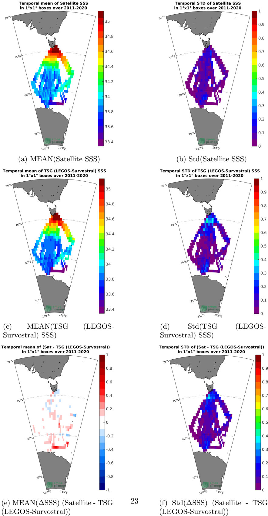
Figure 6: Temporal mean (left) and Std (right) of SSS from SMAP SSS L4 OI v1 - Monthly (IPRC) (top), TSG (LEGOS-Survostral) (middle), and of \Delta SSS (Satellite - TSG (LEGOS-Survostral)). Only match-up pairs are used to generate these maps.
