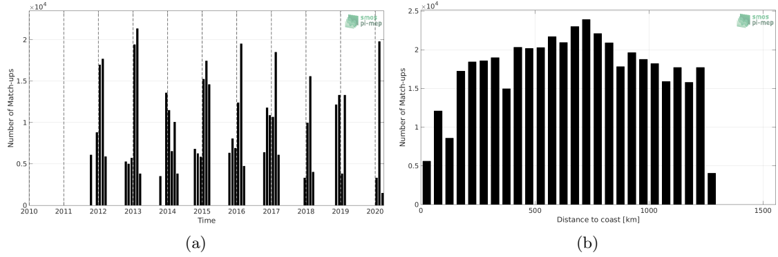
Figure 1: Number of match-ups between TSG (LEGOS-Survostral) and SMAP SSS L4 OI v1 - Monthly (IPRC) SSS as a function of time (a) and as function of the distance to coast (b) over the Global Ocean Pi-MEP region and for the full satellite product period.
