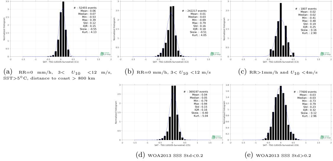
Figure 13: Normalized histogram of \Delta SSS (SMAP SSS L4 OI v1 - Monthly (IPRC) - TSG (LEGOS-Survostral)) for 5 different subdatasets corresponding to: RR=0 mm/h, 3 < U_{10} < 12 m/s, SST>5°C, distance to coast > 800 km (a), RR=0 mm/h, 3 < U_{10} < 12 m/s (b), RR>1mm/h and U_{10} < 4 m/s (c), WOA2013 SSS Std<0.2 (d), WOA2013 SSS Std>0.2 (e).
