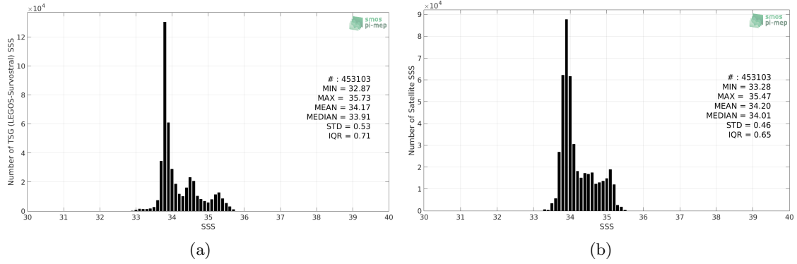
Figure 2: Histograms of SSS from TSG (LEGOS-Survostral) (a) and SMAP SSS L4 OI v1 - Monthly (IPRC) (b) considering all match-up pairs per bins of 0.1 over the Global Ocean Pi-MEP region and for the full satellite product period.
