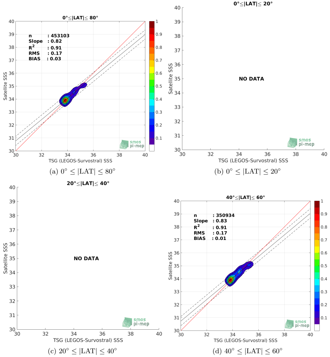
Figure 9: Contour maps of the concentration of SMAP SSS L4 OI v1 - Monthly (IPRC) SSS (y-axis) versus TSG (LEGOS-Survostral) SSS (x-axis) at match-up pairs for different latitude bands. For each plot, the red line shows x=y . The black thin and dashed lines indicate a linear fit through the data cloud and the \pm 95\% confidence levels, respectively. The number match-up pairs n , the slope and R^2 coefficient of the linear fit, the root mean square (RMS) and the mean bias between satellite and in situ data are indicated for each latitude band in each plots.
