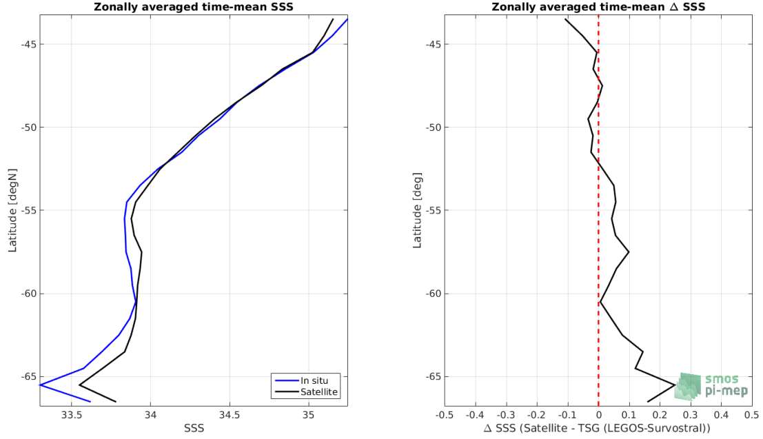
Figure 8: Left panel: Zonal mean SSS from SMAP SSS L4 OI v1 - Monthly (IPRC) satellite product (black) and from TSG (LEGOS-Survostral) (blue). Right panel: Zonal mean of \Delta SSS (Satellite - TSG (LEGOS-Survostral)) for all the collected Pi-MEP match-up pairs estimated over the full satellite product period.
