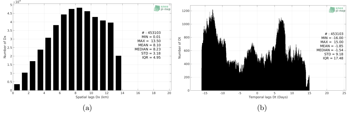
Figure 5: Histograms of the spatial (a) and temporal (b) lags between the location/time of the TSG (LEGOS-Survostral) measurement and the date of the corresponding SMAP SSS L4 OI v1 - Monthly (IPRC) SSS pixel.
