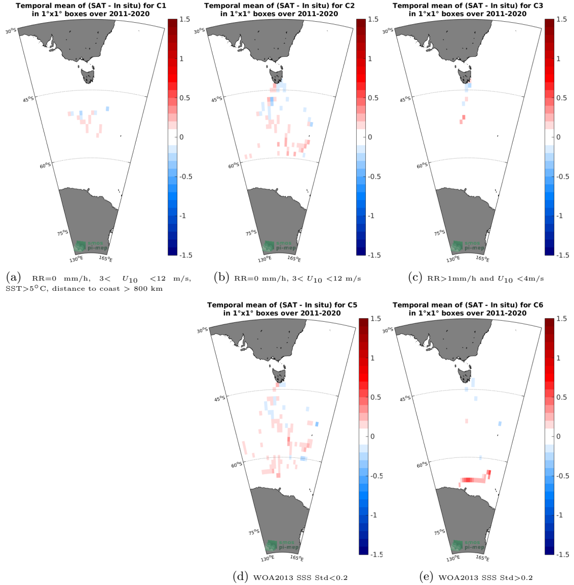
Figure 12: Temporal mean gridded over spatial boxes of size 1^\circ \times 1^\circ of \Delta\text{SSS} (SMAP SSS L4 OI v1 - Monthly (IPRC) - TSG (LEGOS-Survostral)) for 5 different subdatasets corresponding to: RR=0 mm/h, 3 < U_{10} < 12 m/s, SST > 5^\circ\text{C} , distance to coast > 800 km (a), RR=0 mm/h, 3 < U_{10} < 12 m/s (b), RR > 1 mm/h and U_{10} < 4 m/s (c), WOA2013 SSS Std < 0.2 (d), WOA2013 SSS Std > 0.2 (e).
