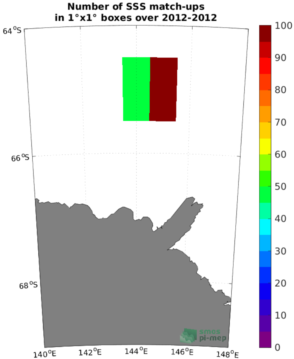
Figure 4: Number of SSS match-ups between TSG (LEGOS-Surv-Adel) SSS and the SMAP SSS L4 OI v1 - Monthly (IPRC) SSS product for the Global Ocean Pi-MEP region over 1^\circ \times 1^\circ boxes and for the full satellite product period.
