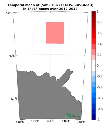
(e) MEAN( \Delta SSS) (Satellite - TSG (LEGOS-Surv-Adel))
