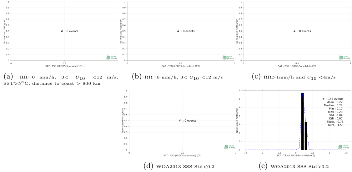
Figure 13: Normalized histogram of \Delta SSS (SMAP SSS L4 OI v1 - Monthly (IPRC) - TSG (LEGOS-Surv-Adel)) for 5 different subdatasets corresponding to: RR=0 mm/h, 3 < U_{10} < 12 m/s, SST > 5°C, distance to coast > 800 km (a), RR=0 mm/h, 3 < U_{10} < 12 m/s (b), RR > 1mm/h and U_{10} < 4 m/s (c), WOA2013 SSS Std < 0.2 (d), WOA2013 SSS Std > 0.2 (e).
