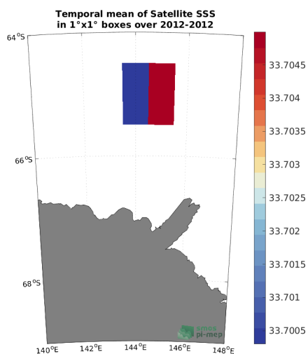
(a) MEAN(Satellite SSS)
