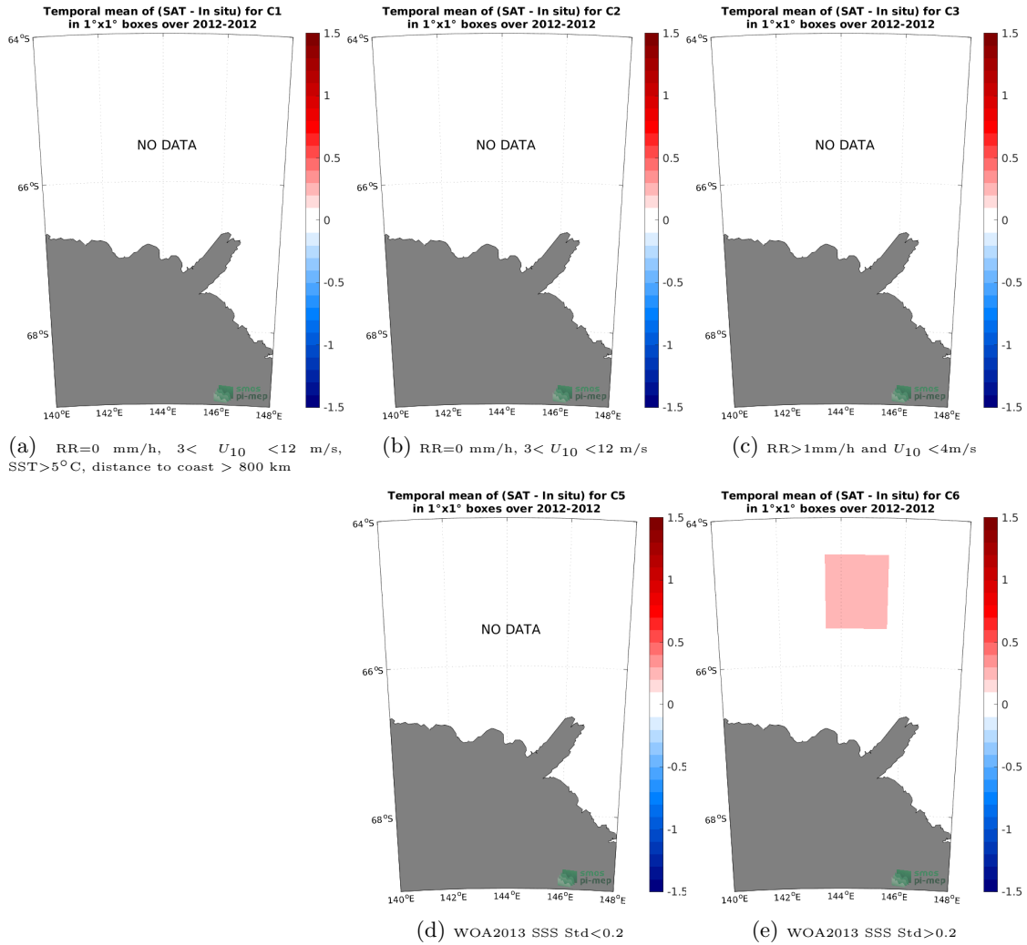
Figure 12: Temporal mean gridded over spatial boxes of size 1^\circ \times 1^\circ of \Delta SSS (SMAP SSS L4 OI v1 - Monthly (IPRC) - TSG (LEGOS-Surv-Adel)) for 5 different subdatasets corresponding to: RR=0 mm/h, 3 < U_{10} < 12 m/s, SST>5°C, distance to coast > 800 km (a), RR=0 mm/h, 3 < U_{10} < 12 m/s (b), RR>1mm/h and U_{10} < 4 m/s (c), WOA2013 SSS Std<0.2 (d), WOA2013 SSS Std>0.2 (e).
