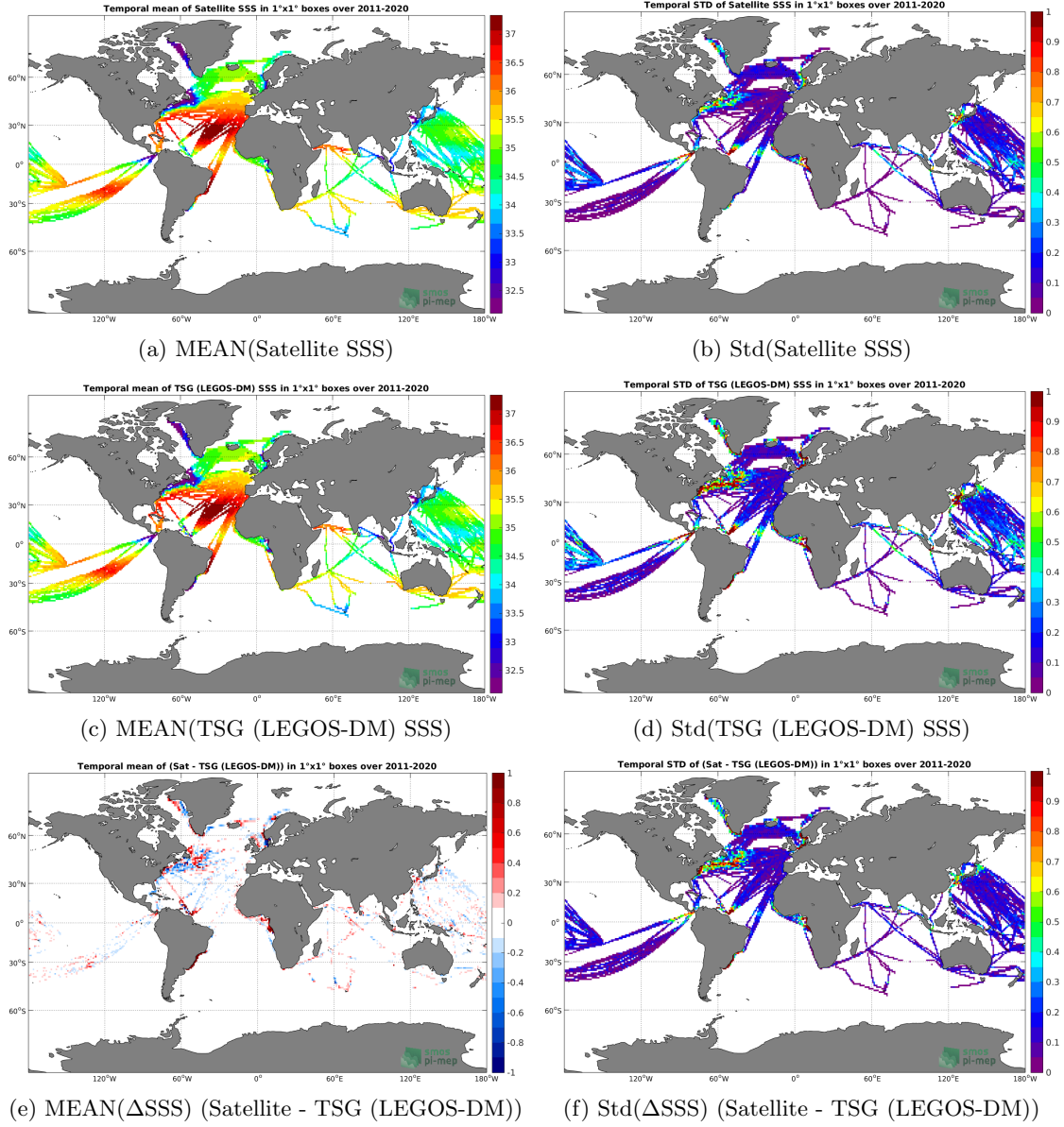
Figure 6: Temporal mean (left) and Std (right) of SSS from SMAP SSS L4 OI v1 - Monthly (IPRC) (top), TSG (LEGOS-DM) (middle), and of \Delta SSS (Satellite - TSG (LEGOS-DM)). Only match-pairs are used to generate these maps.
