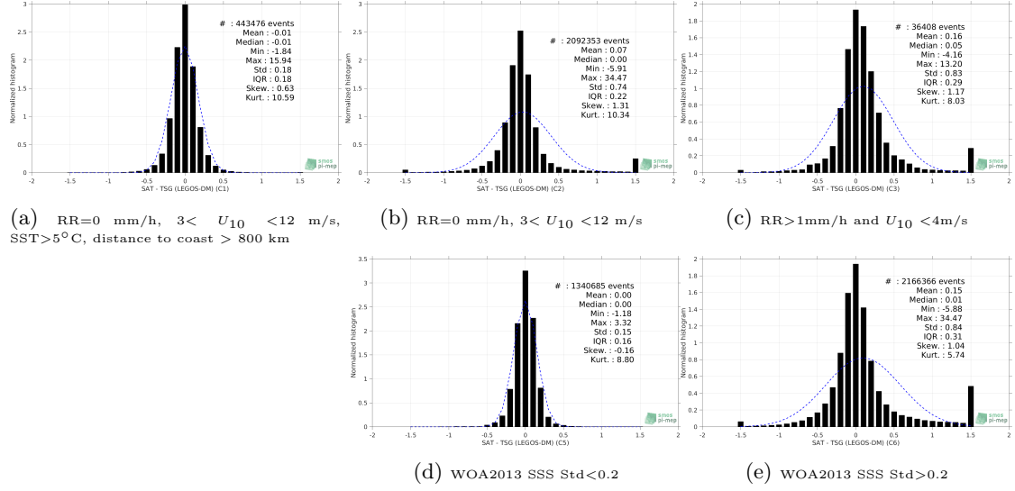
Figure 13: Normalized histogram of \Delta SSS (SMAP SSS L4 OI v1 - Monthly (IPRC) - TSG (LEGOS-DM)) for 5 different subdatasets corresponding to: RR=0 mm/h, 3 < U_{10} < 12 m/s, SST>5°C, distance to coast > 800 km (a), RR=0 mm/h, 3 < U_{10} < 12 m/s (b), RR>1mm/h and U_{10} < 4 m/s (c), WOA2013 SSS Std<0.2 (d), WOA2013 SSS Std>0.2 (e).
