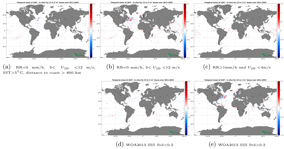
Figure 12: Temporal mean gridded over spatial boxes of size 1^\circ \times 1^\circ of \Delta SSS (SMAP SSS L4 OI v1 - Monthly (IPRC) - TSG (LEGOS-DM)) for 5 different subdatasets corresponding to: RR=0 mm/h, 3 < U_{10} < 12 m/s, SST >5^\circ C, distance to coast > 800 km (a), RR=0 mm/h, 3 < U_{10} < 12 m/s (b), RR >1 mm/h and U_{10} < 4 m/s (c), WOA2013 SSS Std <0.2 (d), WOA2013 SSS Std >0.2 (e).
