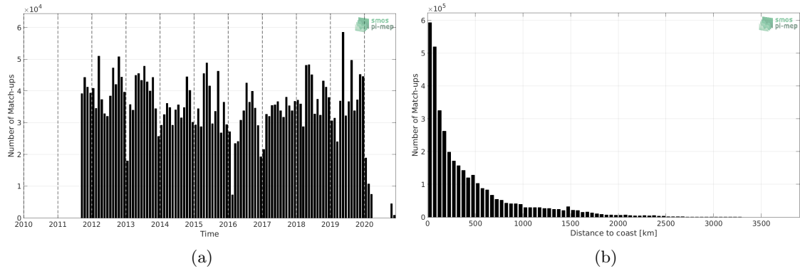
Figure 1: Number of match-ups between TSG (LEGOS-DM) and SMAP SSS L4 OI v1 - Monthly (IPRC) SSS as a function of time (a) and as function of the distance to coast (b) over the Global Ocean Pi-MEP region and for the full satellite product period.
