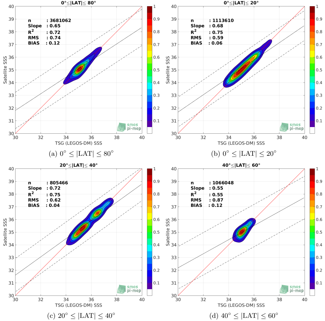
Figure 9: Contour maps of the concentration of SMAP SSS L4 OI v1 - Monthly (IPRC) SSS (y-axis) versus TSG (LEGOS-DM) SSS (x-axis) at match-up pairs for different latitude bands. For each plot, the red line shows x=y . The black thin and dashed lines indicate a linear fit through the data cloud and the \pm 95\% confidence levels, respectively. The number match-up pairs n , the slope and R^2 coefficient of the linear fit, the root mean square (RMS) and the mean bias between satellite and in situ data are indicated for each latitude band in each plots.
