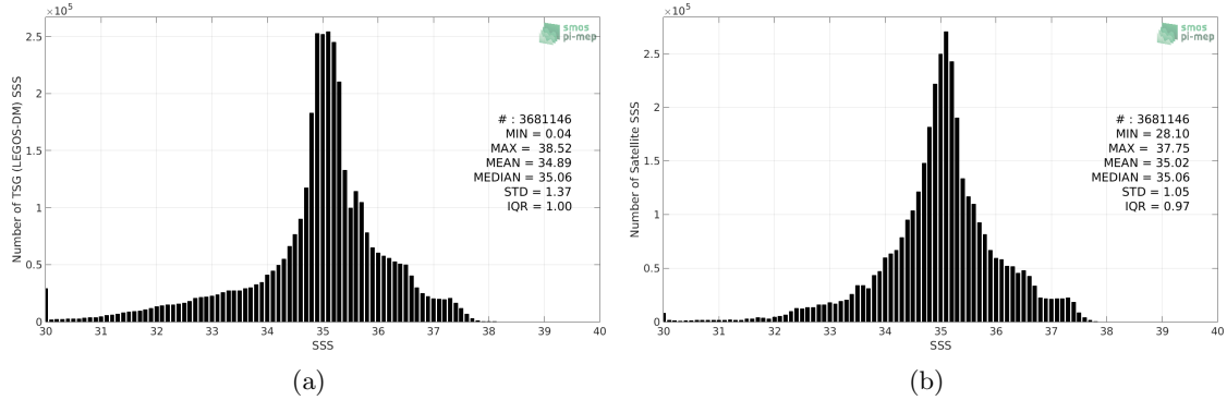
Figure 2: Histograms of SSS from TSG (LEGOS-DM) (a) and SMAP SSS L4 OI v1 - Monthly (IPRC) (b) considering all match-up pairs per bins of 0.1 over the Global Ocean Pi-MEP region and for the full satellite product period.
