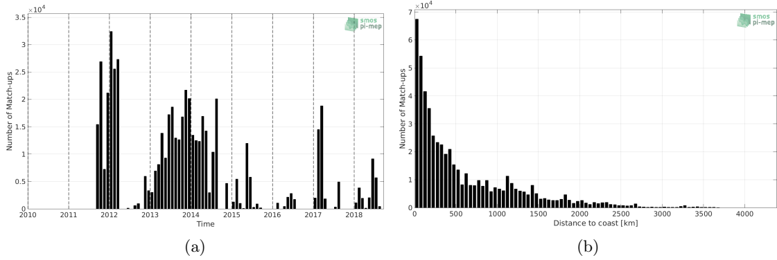
Figure 1: Number of match-ups between TSG (GOSUD-Sailing-ship) and SMAP SSS L4 OI v1 - Monthly (IPRC) SSS as a function of time (a) and as function of the distance to coast (b) over the Global Ocean Pi-MEP region and for the full satellite product period.
