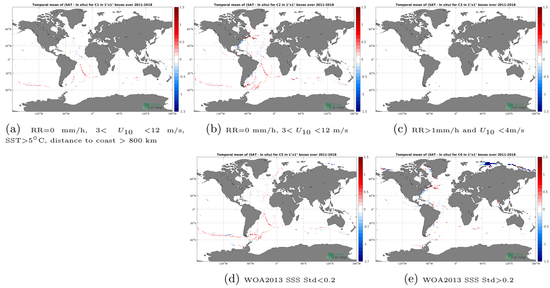
Figure 12: Temporal mean gridded over spatial boxes of size 1^\circ \times 1^\circ of \Delta SSS (SMAP SSS L4 OI v1 - Monthly (IPRC) - TSG (GOSUD-Sailing-ship)) for 5 different subdatasets corresponding to: RR=0 mm/h, 3 < U_{10} < 12 m/s, SST >5^\circ\text{C} , distance to coast > 800 km (a), RR=0 mm/h, 3 < U_{10} < 12 m/s (b), RR >1 mm/h and U_{10} < 4 m/s (c), WOA2013 SSS Std <0.2 (d), WOA2013 SSS Std >0.2 (e).
