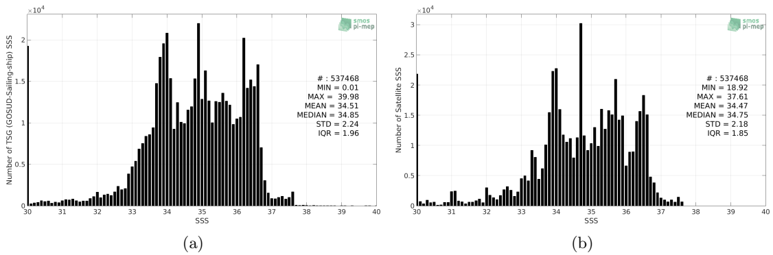
Figure 2: Histograms of SSS from TSG (GOSUD-Sailing-ship) (a) and SMAP SSS L4 OI v1 - Monthly (IPRC) (b) considering all match-up pairs per bins of 0.1 over the Global Ocean Pi-MEP region and for the full satellite product period.
