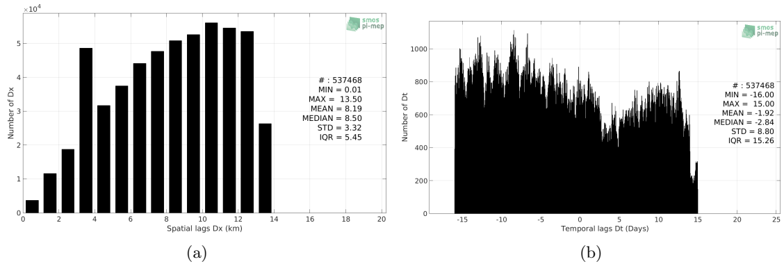
Figure 5: Histograms of the spatial (a) and temporal (b) lags between the location/time of the TSG (GOSUD-Sailing-ship) measurement and the date of the corresponding SMAP SSS L4 OI v1 - Monthly (IPRC) SSS pixel.
