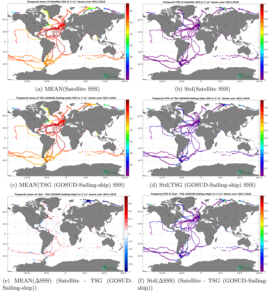
Figure 6: Temporal mean (left) and Std (right) of SSS from SMAP SSS L4 OI v1 - Monthly (IPRC) (top), TSG (GOSUD-Sailing-ship) (middle), and of \Delta SSS (Satellite - TSG (GOSUD-Sailing-ship)). Only match-up pairs are used to generate these maps.
