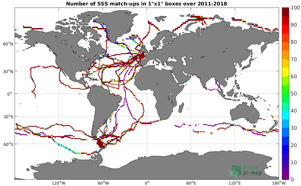
Figure 4: Number of SSS match-ups between TSG (GOSUD-Sailing-ship) SSS and the SMAP SSS L4 OI v1 - Monthly (IPRC) SSS product for the Global Ocean Pi-MEP region over 1^\circ \times 1^\circ boxes and for the full satellite product period.
