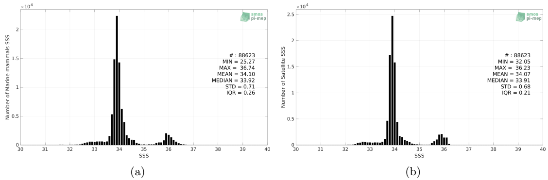
Figure 2: Histograms of SSS from Marine mammals (a) and SMAP SSS L4 OI v1 - Monthly (IPRC) (b) considering all match-up pairs per bins of 0.1 over the Global Ocean Pi-MEP region and for the full satellite product period.
