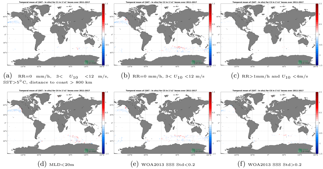
Figure 12: Temporal mean gridded over spatial boxes of size 1^\circ \times 1^\circ of \Delta SSS (SMAP SSS L4 OI v1 - Monthly (IPRC) - Marine mammals) for 6 different subdatasets corresponding to:RR=0 mm/h, 3 < U_{10} < 12 m/s, SST >5^\circ\text{C} , distance to coast > 800 km (a), RR=0 mm/h, 3 < U_{10} < 12 m/s (b), RR >1 mm/h and U_{10} < 4 m/s (c),MLD <20 m (d),WOA2013 SSS Std <0.2 (e),WOA2013 SSS Std >0.2 (f).
