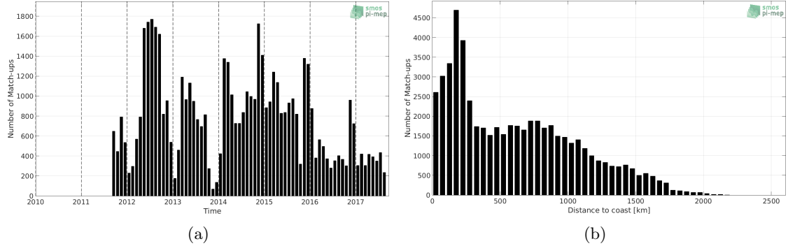
Figure 1: Number of match-ups between Marine mammals and SMAP SSS L4 OI v1 - Monthly (IPRC) SSS as a function of time (a) and as function of the distance to coast (b) over the Global Ocean Pi-MEP region and for the full satellite product period.
