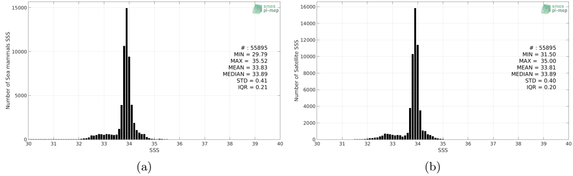
Figure 2: Histograms of SSS from Marine mammals (a) and SMAP SSS L4 OI v1 - Monthly (IPRC) (b) considering all match-up pairs per bins of 0.1 over the Global Ocean Pi-MEP region and for the full satellite product period.
