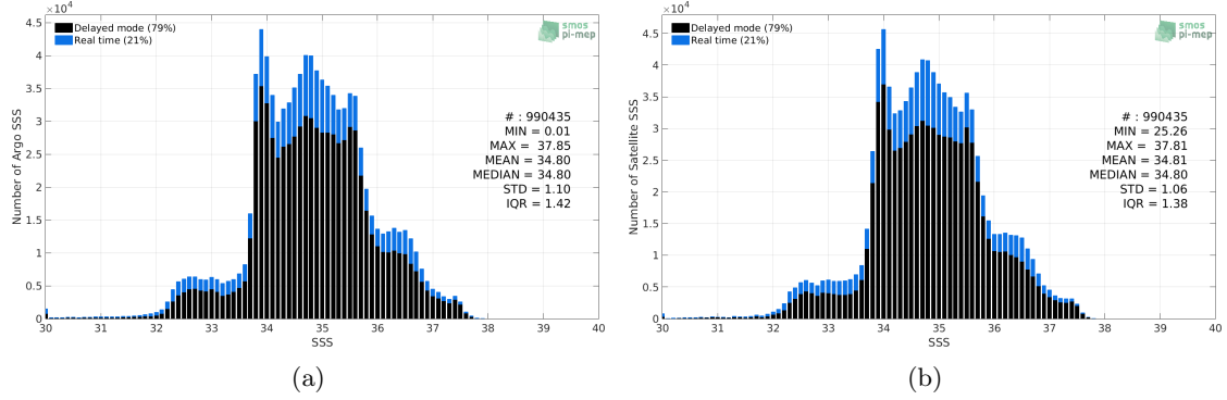
Figure 2: Histograms of SSS from Argo (a) and SMAP SSS L4 OI v1 - Monthly (IPRC) (b) considering all match-up pairs per bins of 0.1 over the Global Ocean Pi-MEP region and for the full satellite product period.
