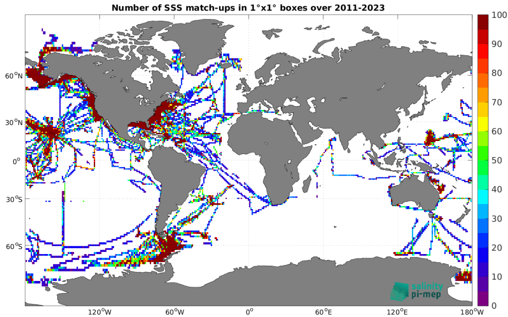
Figure 5: Number of SSS match-ups between TSG (SAMOS) SSS and the SMAP SSS L4 OI v3 - Monthly (ESR) SSS product for the Global Ocean Pi-MEP region over 1^\circ \times 1^\circ boxes and for the full satellite product period.
