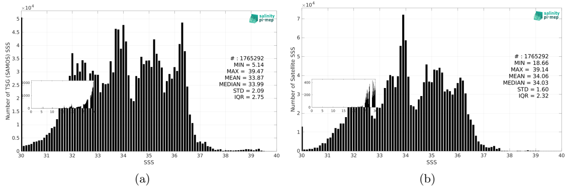
Figure 3: Histograms of SSS from TSG (SAMOS) (a) and SMAP SSS L4 OI v3 - Monthly (ESR) (b) considering all match-up pairs per bins of 0.1 over the Global Ocean Pi-MEP region and for the full satellite product period.
