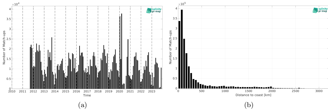
Figure 2: Number of match-ups between TSG (SAMOS) and SMAP SSS L4 OI v3 - Monthly (ESR) SSS as a function of time (a) and as function of the distance to coast (b) over the Global Ocean Pi-MEP region and for the full satellite product period.
