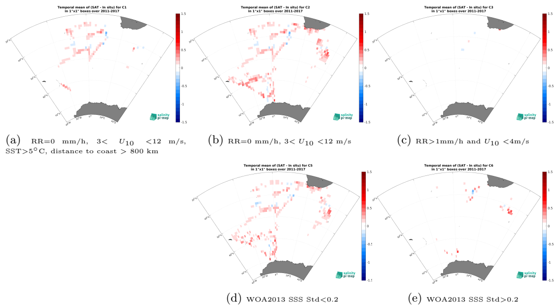
Figure 14: Temporal mean gridded over spatial boxes of size 1^\circ \times 1^\circ of \Delta SSS (SMAP SSS L4 OI v3 - Monthly (ESR) - TSG (NCEI-0170743)) for 5 different subdatasets corresponding to:RR=0 mm/h, 3 < U_{10} < 12 m/s, SST >5^\circ\text{C} , distance to coast > 800 km (a), RR=0 mm/h, 3 < U_{10} < 12 m/s (b), RR >1 mm/h and U_{10} < 4 m/s (c), WOA2013 SSS Std <0.2 (d), WOA2013 SSS Std >0.2 (e).
