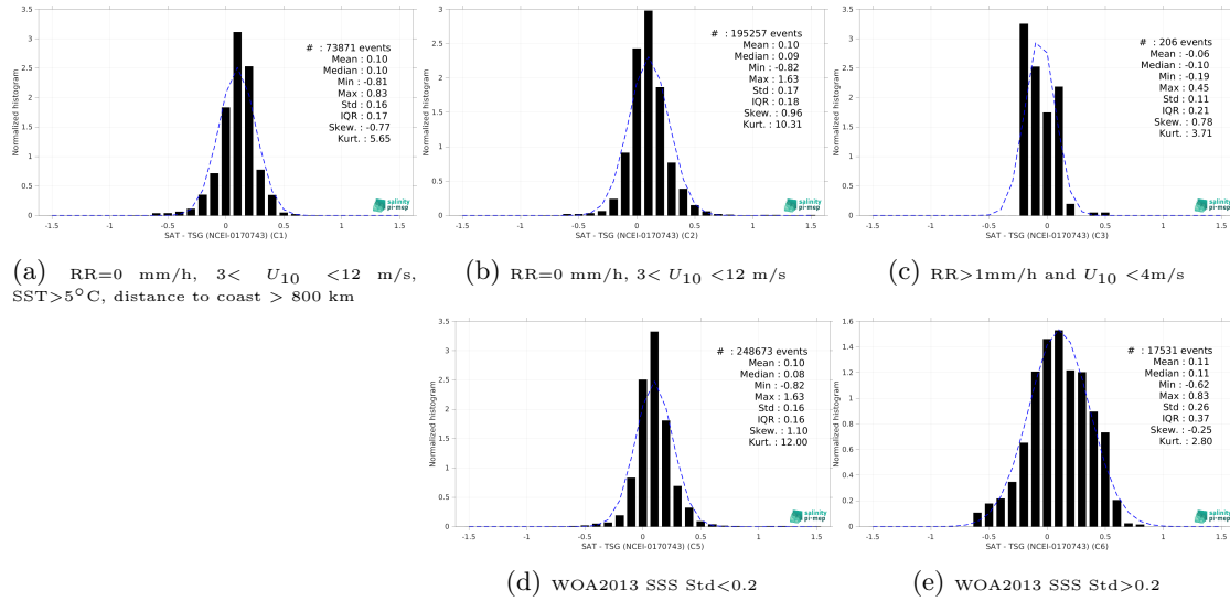
Figure 15: Normalized histogram of \Delta\text{SSS} (SMAP SSS L4 OI v3 - Monthly (ESR) - TSG (NCEI-0170743)) for 5 different subdatasets corresponding to: RR=0 mm/h, 3 < U_{10} < 12 m/s, SST>5°C, distance to coast > 800 km (a), RR=0 mm/h, 3 < U_{10} < 12 m/s (b), RR>1mm/h and U_{10} < 4 m/s (c), WOA2013 SSS Std<0.2 (d), WOA2013 SSS Std>0.2 (e).
