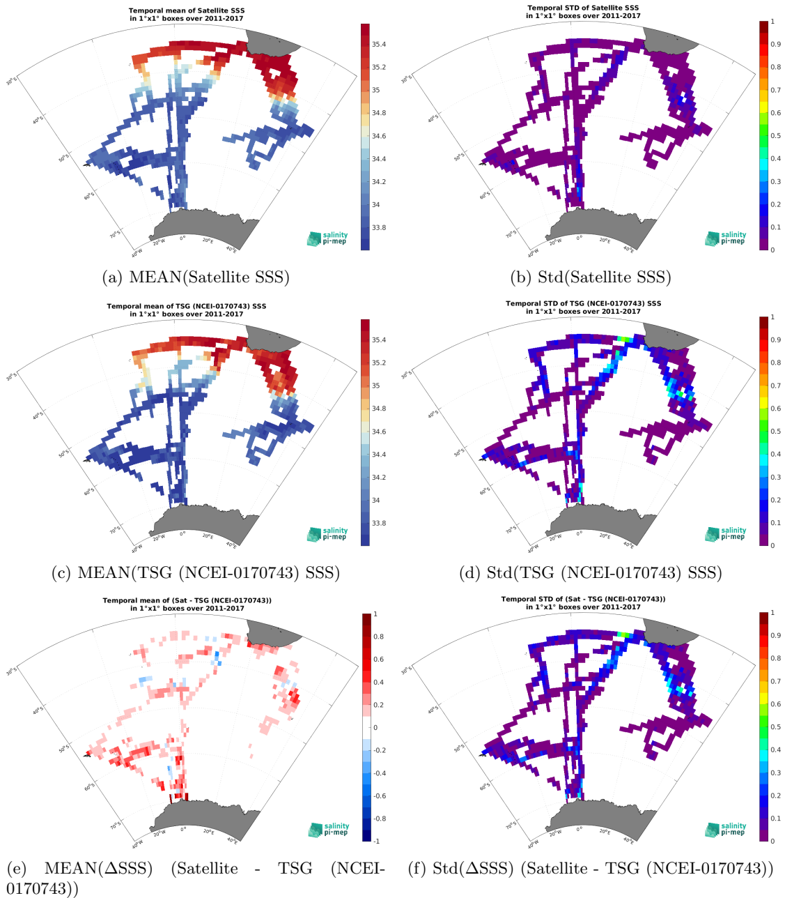
Figure 7: Temporal mean (left) and Std (right) of SSS from SMAP SSS L4 OI v3 - Monthly (ESR) (top), TSG (NCEI-0170743) (middle), and of \Delta SSS (Satellite - TSG (NCEI-0170743)). Only match-up pairs are used to generate these maps.
