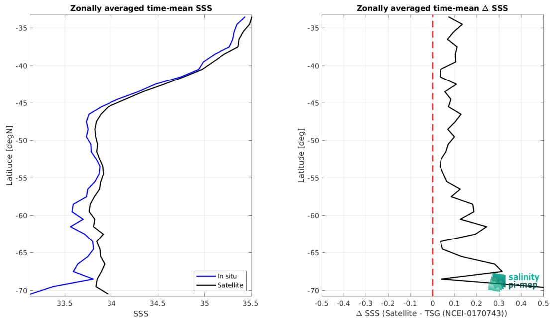
Figure 9: Left panel: Zonal mean SSS from SMAP SSS L4 OI v3 - Monthly (ESR) satellite product (black) and from TSG (NCEI-0170743) (blue). Right panel: Zonal mean of \Delta SSS (Satellite - TSG (NCEI-0170743)) for all the collected Pi-MEP match-up pairs estimated over the full satellite product period.
