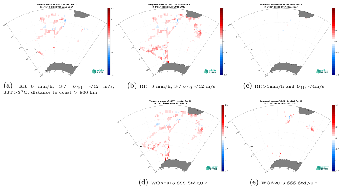
Figure 14: Temporal mean gridded over spatial boxes of size 1^\circ \times 1^\circ of \Delta\text{SSS} (SMAP SSS L4 OI v3 - Monthly (ESR) - TSG (NCEI-0170743)) for 5 different subdatasets corresponding to:RR=0 mm/h, 3 < U_{10} < 12 m/s, SST>5°C, distance to coast > 800 km (a), RR=0 mm/h, 3 < U_{10} < 12 m/s (b), RR>1mm/h and U_{10} < 4 m/s (c), WOA2013 SSS Std<0.2 (d), WOA2013 SSS Std>0.2 (e).
