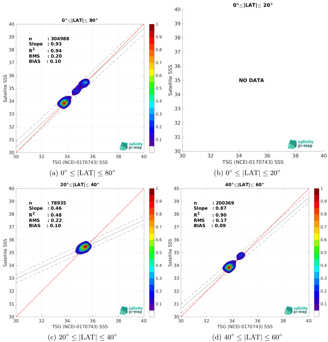
Figure 10: Contour maps of the concentration of SMAP SSS L4 OI v3 - Monthly (ESR) SSS (y-axis) versus TSG (NCEI-0170743) SSS (x-axis) at match-up pairs for different latitude bands. For each plot, the red line shows x=y . The black thin and dashed lines indicate a linear fit through the data cloud and the \pm 95\% confidence levels, respectively. The number match-up pairs n , the slope and R^2 coefficient of the linear fit, the root mean square (RMS) and the mean bias between satellite and in situ data are indicated for each latitude band in each plots.
