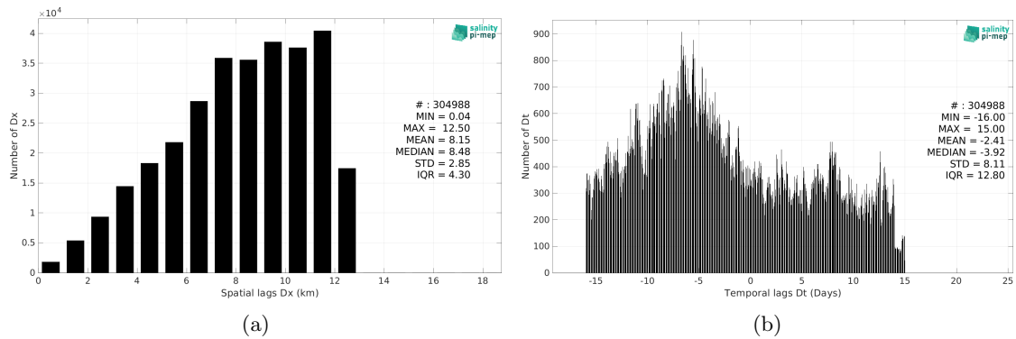
Figure 6: Histograms of the spatial (a) and temporal (b) lags between the location/time of the TSG (NCEI-0170743) measurement and the date of the corresponding SMAP SSS L4 OI v3 - Monthly (ESR) SSS pixel.
