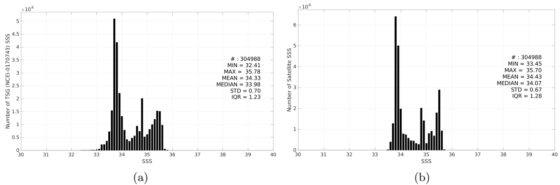
Figure 3: Histograms of SSS from TSG (NCEI-0170743) (a) and SMAP SSS L4 OI v3 - Monthly (ESR) (b) considering all match-up pairs per bins of 0.1 over the Global Ocean Pi-MEP region and for the full satellite product period.
