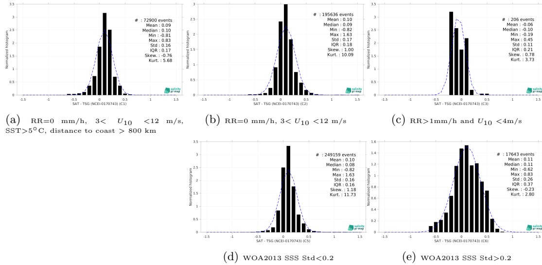
Figure 15: Normalized histogram of \Delta SSS (SMAP SSS L4 OI v3 - Monthly (ESR) - TSG (NCEI-0170743)) for 5 different subdatasets corresponding to: RR=0 mm/h, 3 < U_{10} < 12 m/s, SST > 5°C, distance to coast > 800 km (a), RR=0 mm/h, 3 < U_{10} < 12 m/s (b), RR > 1mm/h and U_{10} < 4 m/s (c), WOA2013 SSS Std < 0.2 (d), WOA2013 SSS Std > 0.2 (e).
