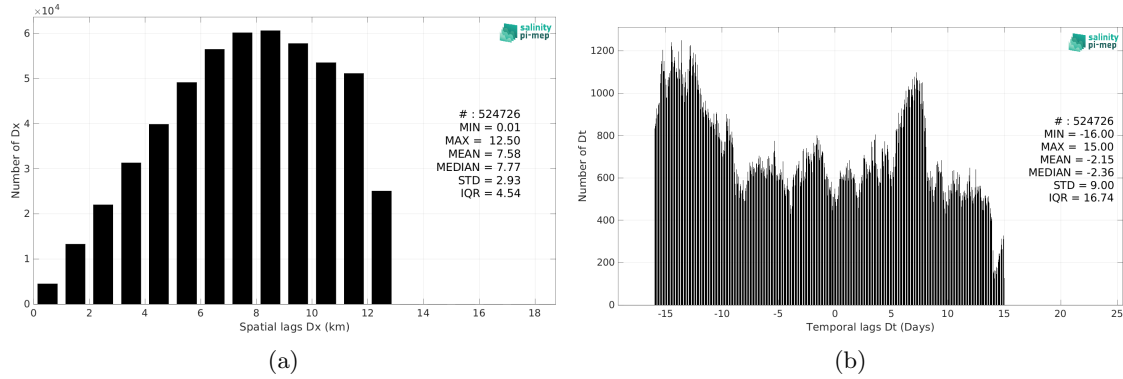
Figure 6: Histograms of the spatial (a) and temporal (b) lags between the location/time of the TSG (LEGOS-Survostral) measurement and the date of the corresponding SMAP SSS L4 OI v3 - Monthly (ESR) SSS pixel.
