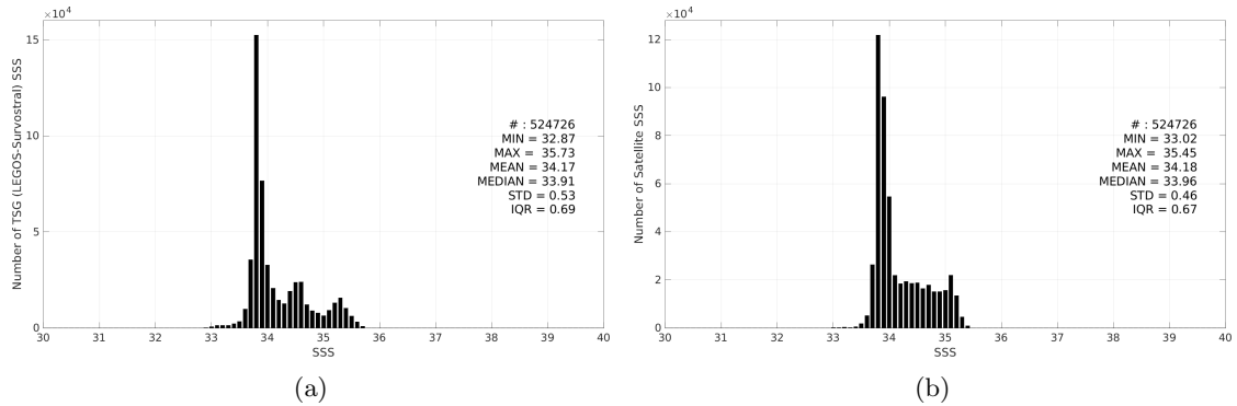
Figure 3: Histograms of SSS from TSG (LEGOS-Survostral) (a) and SMAP SSS L4 OI v3 - Monthly (ESR) (b) considering all match-up pairs per bins of 0.1 over the Global Ocean Pi-MEP region and for the full satellite product period.
