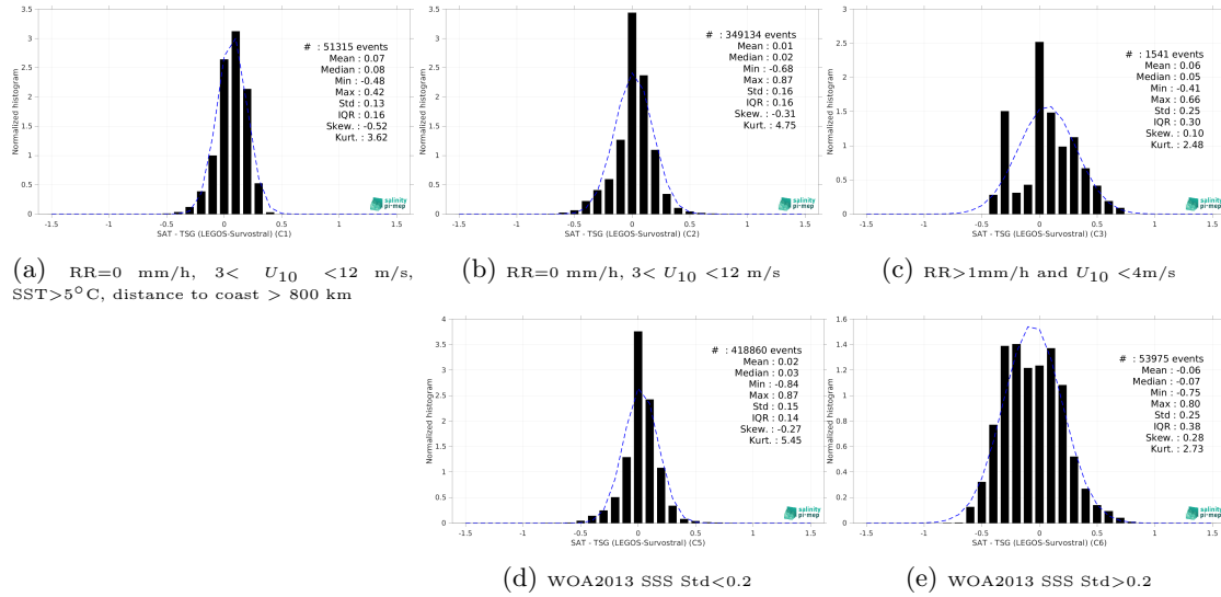
Figure 15: Normalized histogram of \Delta SSS (SMAP SSS L4 OI v3 - Monthly (ESR) - TSG (LEGOs-Survostral)) for 5 different subdatasets corresponding to: RR=0 mm/h, 3 < U_{10} < 12 m/s, SST > 5°C, distance to coast > 800 km (a), RR=0 mm/h, 3 < U_{10} < 12 m/s (b), RR > 1mm/h and U_{10} < 4 m/s (c), WOA2013 SSS Std < 0.2 (d), WOA2013 SSS Std > 0.2 (e).
