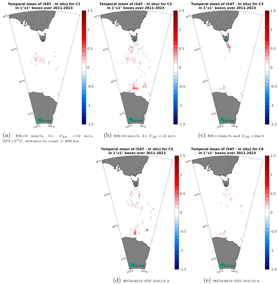
Figure 14: Temporal mean gridded over spatial boxes of size 1^\circ \times 1^\circ of \Delta SSS (SMAP SSS L4 OI v3 - Monthly (ESR) - TSG (LEGOS-Survostral)) for 5 different subdatasets corresponding to: RR=0 mm/h, 3 < U_{10} < 12 m/s, SST>5°C, distance to coast > 800 km (a), RR=0 mm/h, 3 < U_{10} < 12 m/s (b), RR>1mm/h and U_{10} < 4 m/s (c), WOA2013 SSS Std<0.2 (d), WOA2013 SSS Std>0.2 (e).
