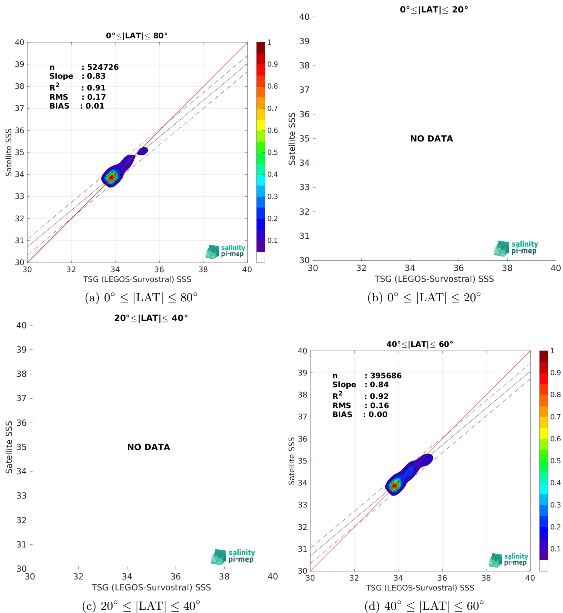
Figure 10: Contour maps of the concentration of SMAP SSS L4 OI v3 - Monthly (ESR) SSS (y-axis) versus TSG (LEGOS-Survostral) SSS (x-axis) at match-up pairs for different latitude bands. For each plot, the red line shows x=y . The black thin and dashed lines indicate a linear fit through the data cloud and the \pm 95\% confidence levels, respectively. The number match-up pairs n , the slope and R^2 coefficient of the linear fit, the root mean square (RMS) and the mean bias between satellite and in situ data are indicated for each latitude band in each plots.
