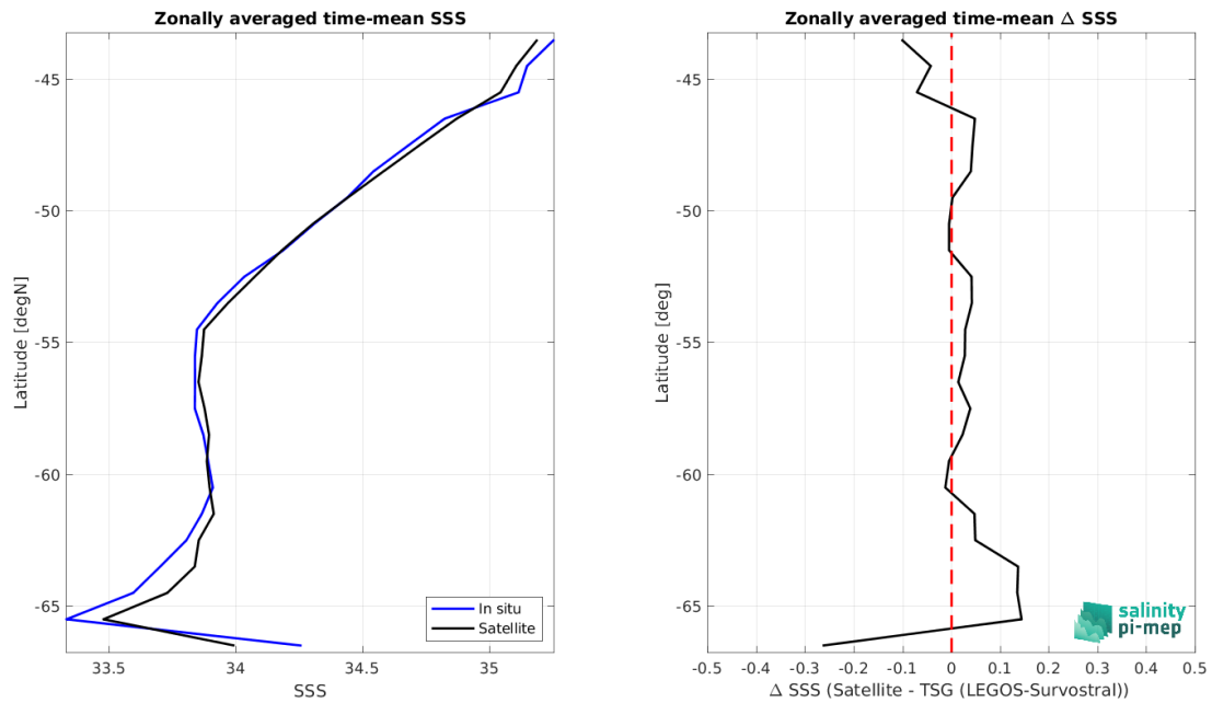
Figure 9: Left panel: Zonal mean SSS from SMAP SSS L4 OI v3 - Monthly (ESR) satellite product (black) and from TSG (LEGOS-Survostral) (blue). Right panel: Zonal mean of \Delta SSS (Satellite - TSG (LEGOS-Survostral)) for all the collected Pi-MEP match-up pairs estimated over the full satellite product period.
