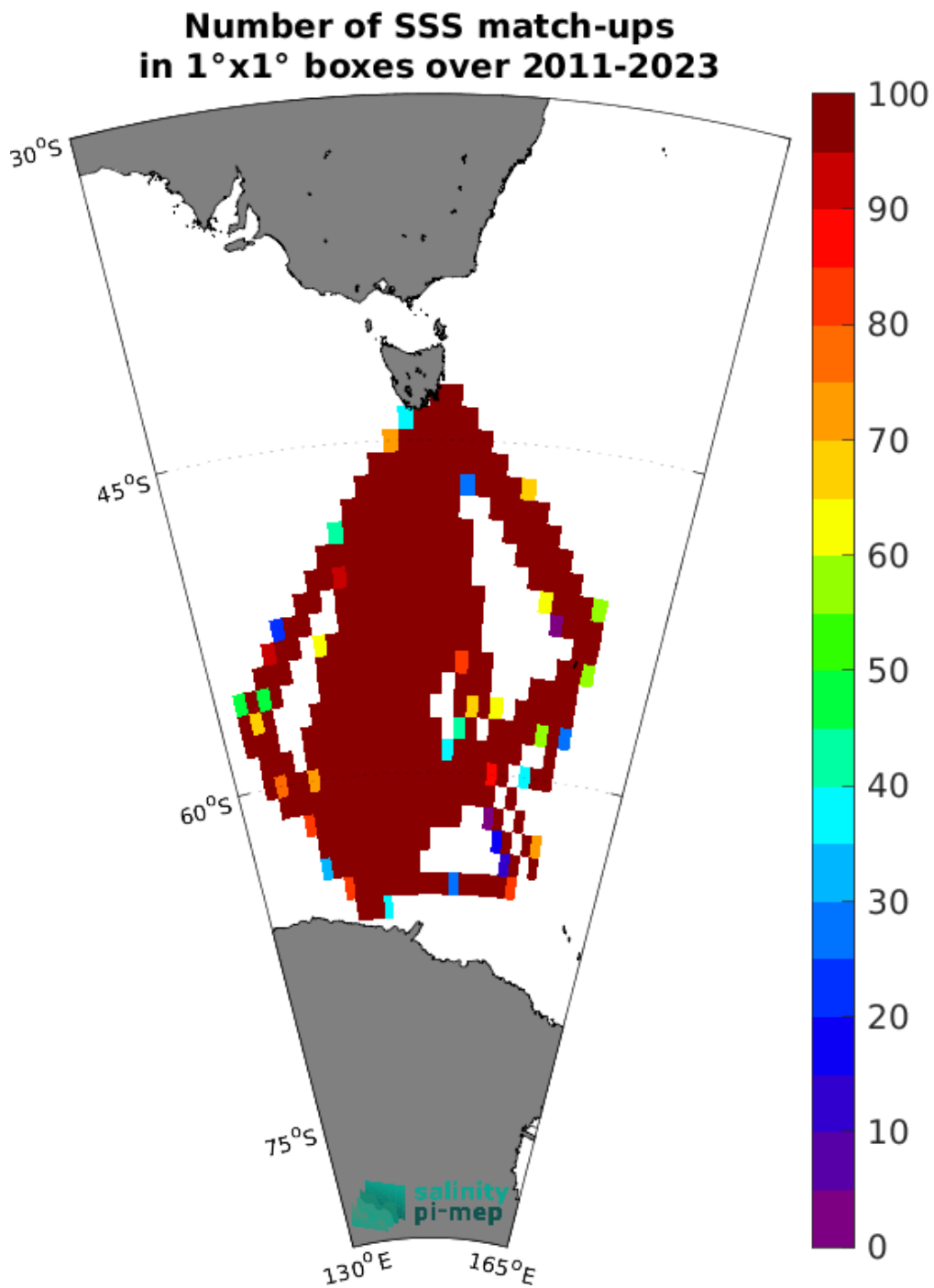
Figure 5: Number of SSS match-ups between TSG (LEGOS-Survostral) SSS and the SMAP SSS L4 OI v3 - Monthly (ESR) SSS product for the Global Ocean Pi-MEP region over 1°x1° boxes and for the full satellite product period.
