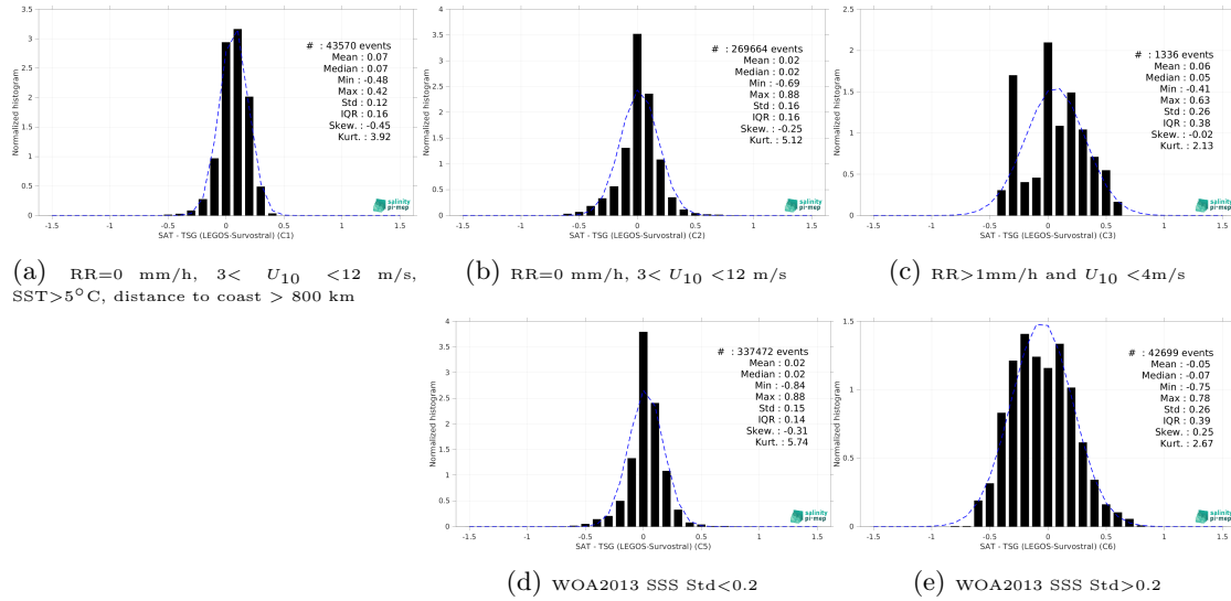
Figure 15: Normalized histogram of \Delta SSS (SMAP SSS L4 OI v3 - Monthly (ESR) - TSG (LEGOS-Survostral)) for 5 different subdatasets corresponding to: RR=0 mm/h, 3 < U_{10} < 12 m/s, SST>5°C, distance to coast > 800 km (a), RR=0 mm/h, 3 < U_{10} < 12 m/s (b), RR>1mm/h and U_{10} < 4 m/s (c), WOA2013 SSS Std<0.2 (d), WOA2013 SSS Std>0.2 (e).
