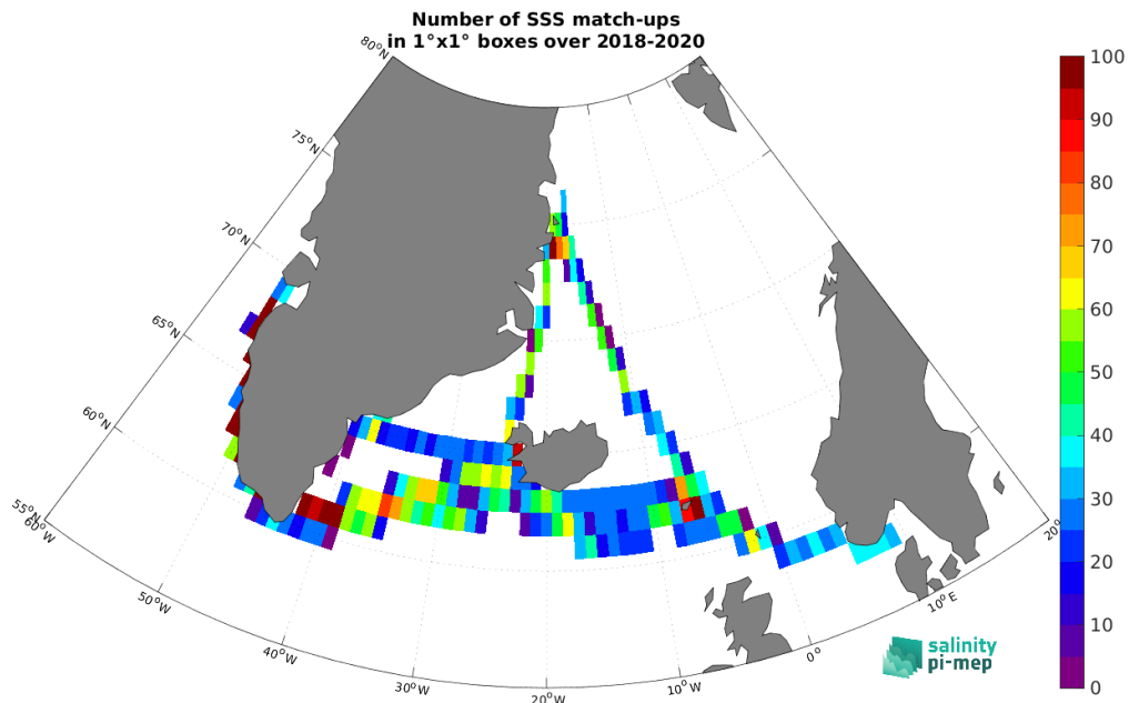
Figure 5: Number of SSS match-ups between TSG (Lauge-Koch) SSS and the SMAP SSS L4 OI v3 - Monthly (ESR) SSS product for the Global Ocean Pi-MEP region over 1^\circ \times 1^\circ boxes and for the full satellite product period.
