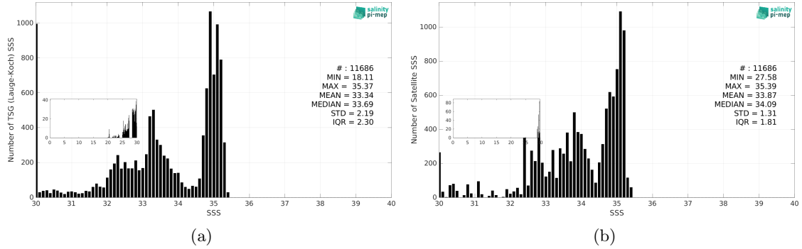
Figure 3: Histograms of SSS from TSG (Lauge-Koch) (a) and SMAP SSS L4 OI v3 - Monthly (ESR) (b) considering all match-up pairs per bins of 0.1 over the Global Ocean Pi-MEP region and for the full satellite product period.
