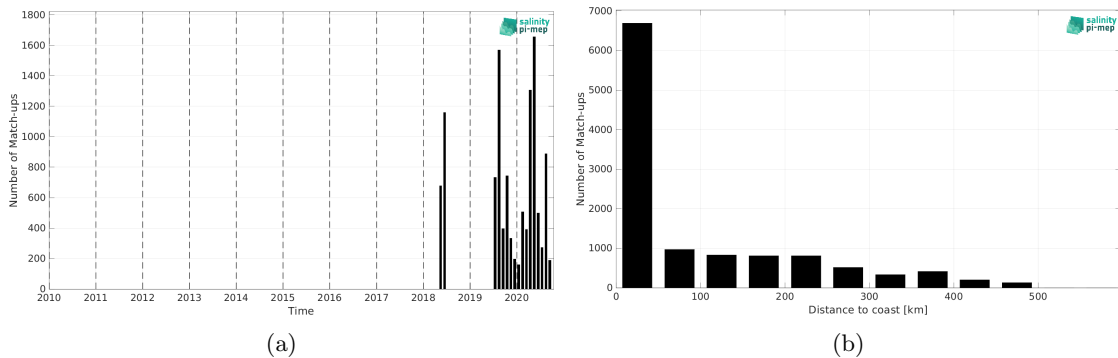
Figure 2: Number of match-ups between TSG (Lauge-Koch) and SMAP SSS L4 OI v3 - Monthly (ESR) SSS as a function of time (a) and as function of the distance to coast (b) over the Global Ocean Pi-MEP region and for the full satellite product period.
