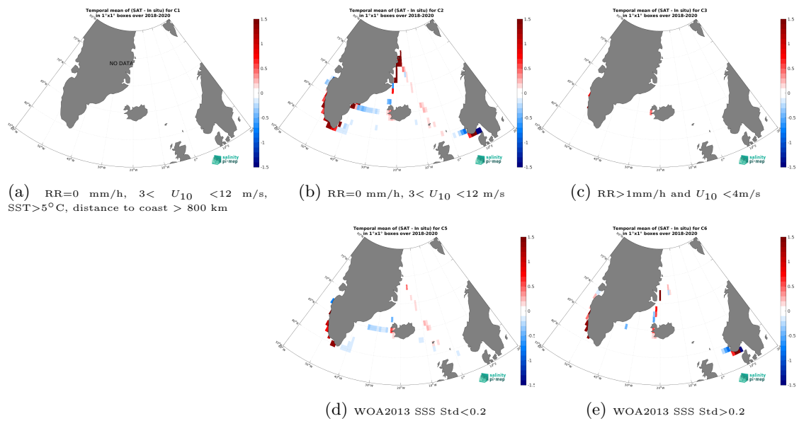
Figure 14: Temporal mean gridded over spatial boxes of size 1^\circ \times 1^\circ of \Delta\text{SSS} (SMAP SSS L4 OI v3 - Monthly (ESR) - TSG (Lauge-Koch)) for 5 different subdatasets corresponding to: RR=0 mm/h, 3 < U_{10} < 12 m/s, SST > 5^\circ\text{C} , distance to coast > 800 km (a), RR=0 mm/h, 3 < U_{10} < 12 m/s (b), RR > 1 mm/h and U_{10} < 4 m/s (c), WOA2013 SSS Std < 0.2 (d), WOA2013 SSS Std > 0.2 (e).
