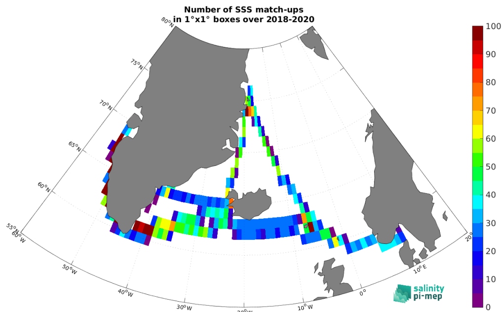
Figure 5: Number of SSS match-ups between TSG (Lauge-Koch) SSS and the SMAP SSS L4 OI v3 - Monthly (ESR) SSS product for the Global Ocean Pi-MEP region over 1^\circ \times 1^\circ boxes and for the full satellite product period.
