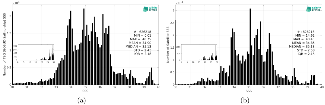
Figure 3: Histograms of SSS from TSG (GOSUD-Sailing-ship) (a) and SMAP SSS L4 OI v3 - Monthly (ESR) (b) considering all match-up pairs per bins of 0.1 over the Global Ocean Pi-MEP region and for the full satellite product period.
