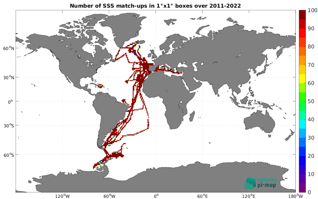
Figure 5: Number of SSS match-ups between TSG (CSIC-UTM) SSS and the SMAP SSS L4 OI v3 - Monthly (ESR) SSS product for the Global Ocean Pi-MEP region over 1^\circ \times 1^\circ boxes and for the full satellite product period.
