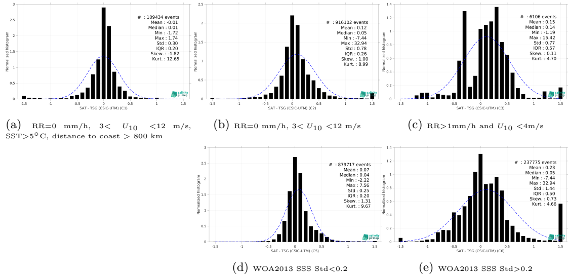
Figure 15: Normalized histogram of \Delta\text{SSS} (SMAP SSS L4 OI v3 - Monthly (ESR) - TSG (CSIC-UTM)) for 5 different subdatasets corresponding to: RR=0 mm/h, 3 < U_{10} < 12 m/s, SST > 5^\circ\text{C} , distance to coast > 800 km (a), RR=0 mm/h, 3 < U_{10} < 12 m/s (b), RR > 1 mm/h and U_{10} < 4 m/s (c), WOA2013 SSS Std < 0.2 (d), WOA2013 SSS Std > 0.2 (e).
