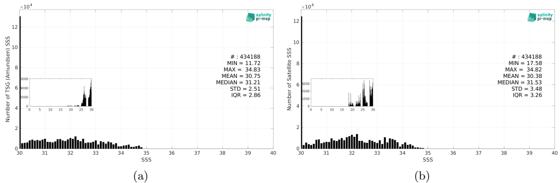
Figure 3: Histograms of SSS from TSG (Amundsen) (a) and SMAP SSS L4 OI v3 - Monthly (ESR) (b) considering all match-up pairs per bins of 0.1 over the Global Ocean Pi-MEP region and for the full satellite product period.
