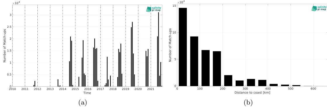
Figure 2: Number of match-ups between TSG (Amundsen) and SMAP SSS L4 OI v3 - Monthly (ESR) SSS as a function of time (a) and as function of the distance to coast (b) over the Global Ocean Pi-MEP region and for the full satellite product period.
